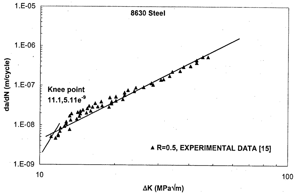
Figure A27. Knee point used to find \rho^* for R=0.5, 8630 cast steel [15].
