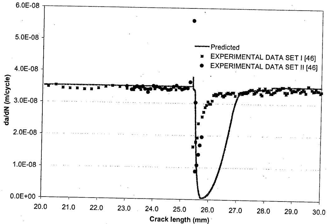
Figure 47. Crack growth retardation due to overload predicted using the residual K approach for 4140 Steel.
