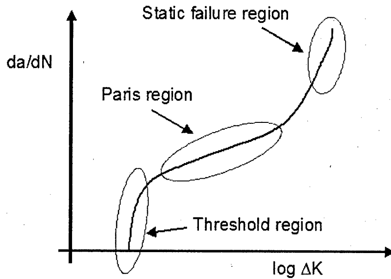
Figure 7. Illustration of fatigue crack growth rate curve.
