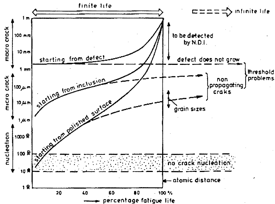
Figure 2. A simple representation of different crack growth cases [2]
