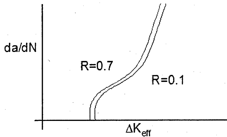
Figure 13. Expected theoretical correlation using the K_{eff} method.
