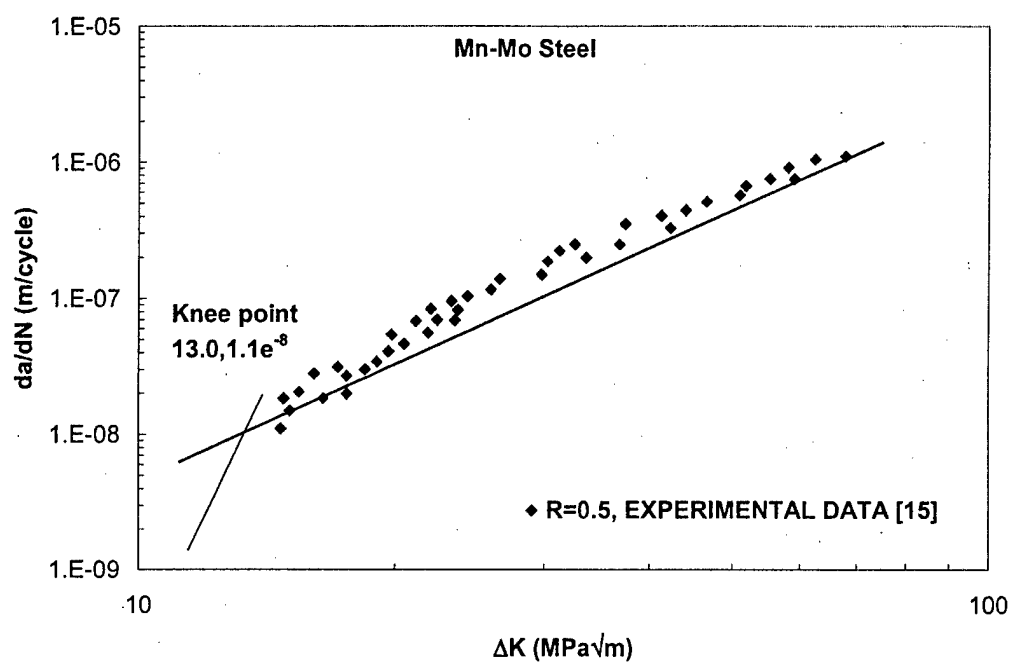
Figure A23. Knee point used to find \rho^* for R=0.5 , Mn-Mo cast steel [15].
