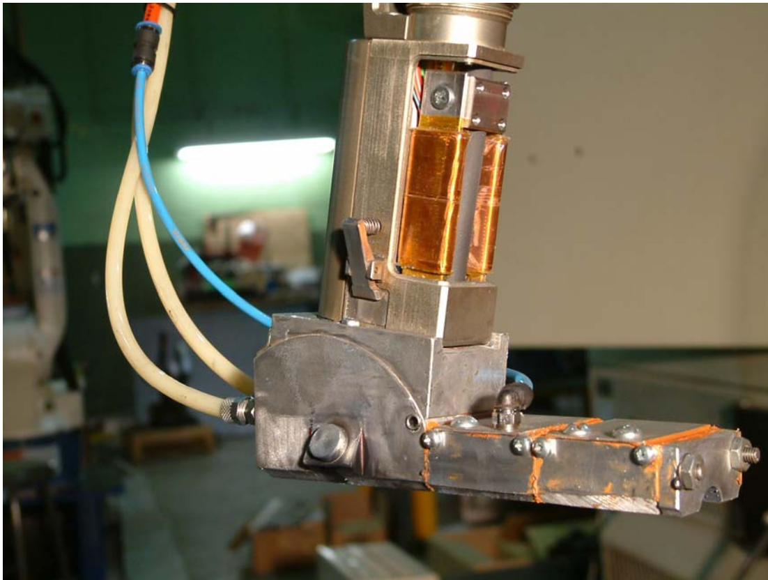
Fig.5 Magnetic device placed in SMIG Torch Body. (Copper attachment)
