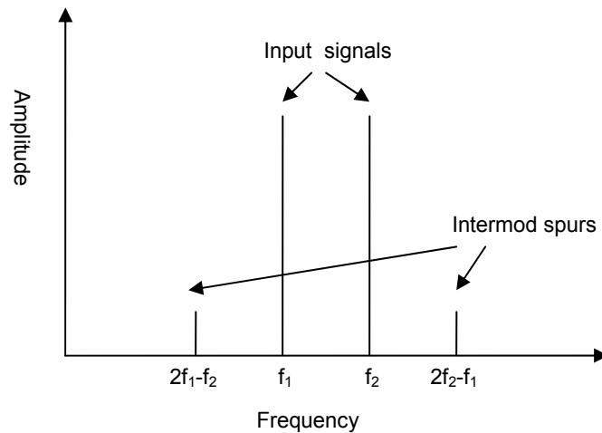
Figure 2-7 Third-order intermodulation products with associated frequency components, plotted frequency vs. amplitude, reproduced from (Tsui, 2001:224).
