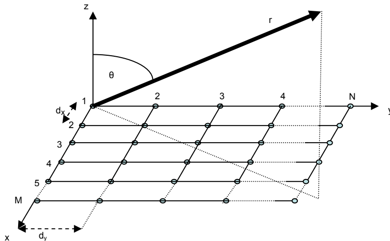
Figure 2-2 Geometry of a planar array used to derive the array factor, reproduced from (Balanis, 1997:310).
