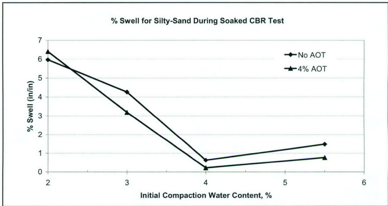
Figure 49. Swelling response on silty-sand during soaked CBR test
