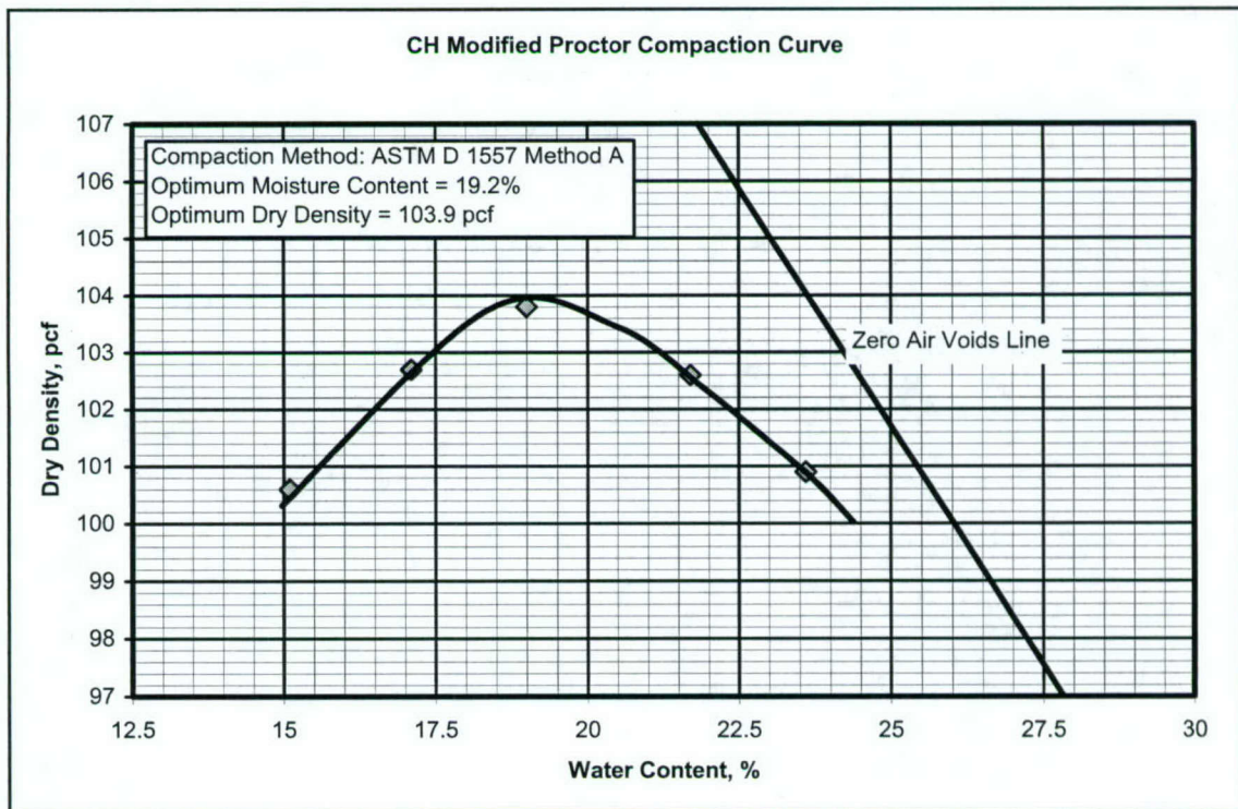
Figure 22. Modified proctor compaction curve for CH
