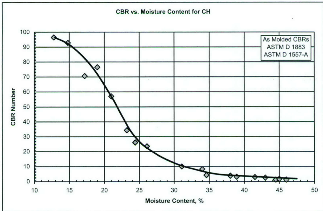
Figure 25. CBR versus moisture content curve for CH
