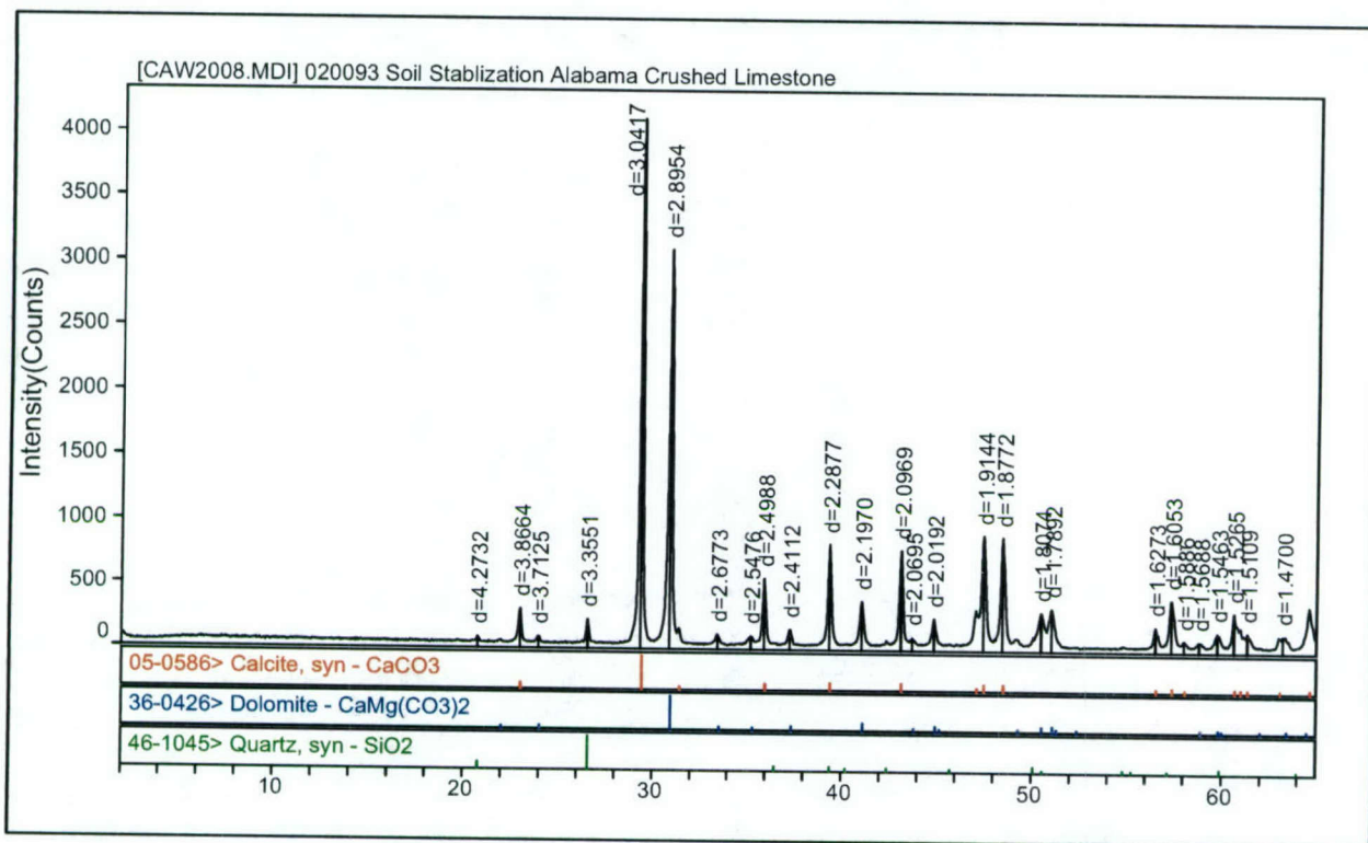
Figure 9. X-ray diffraction pattern of limestone dust
