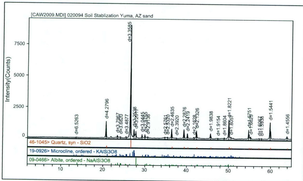
Figure 10. X-ray diffraction pattern of Yuma sand comprised primarily of quartz and feldspar
