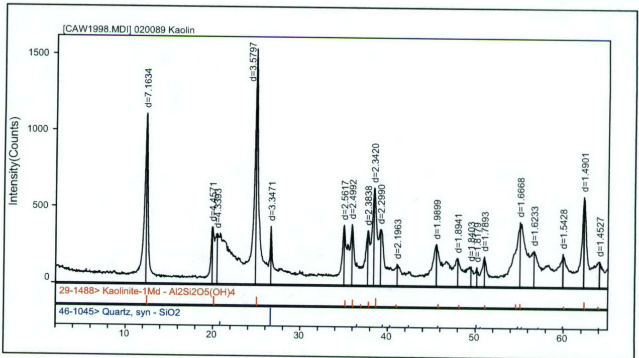
Figure 4. X-ray diffraction pattern of kaolinite
