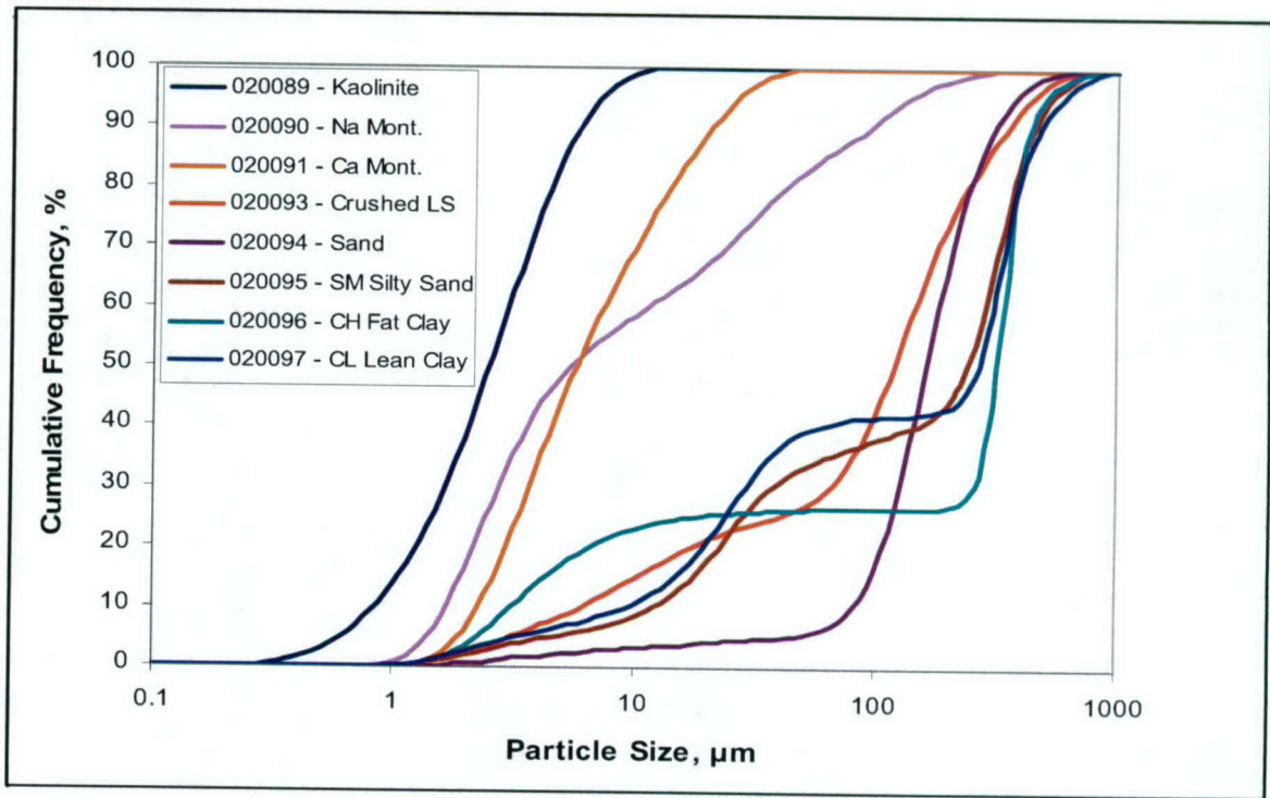
Figure 3. Cumulative log-scale particle size distribution analysis of minerals
