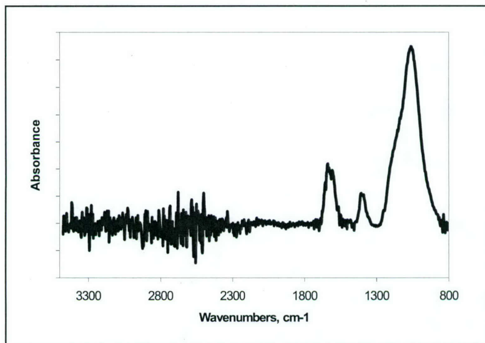
Figure 29. FTIR/ATR spectrum of Ven-Set 950 soil stabilization agent
