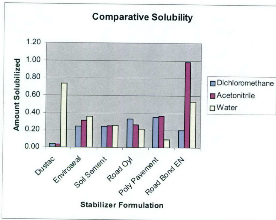
Figure 35. Comparative solubility of stabilization agents
