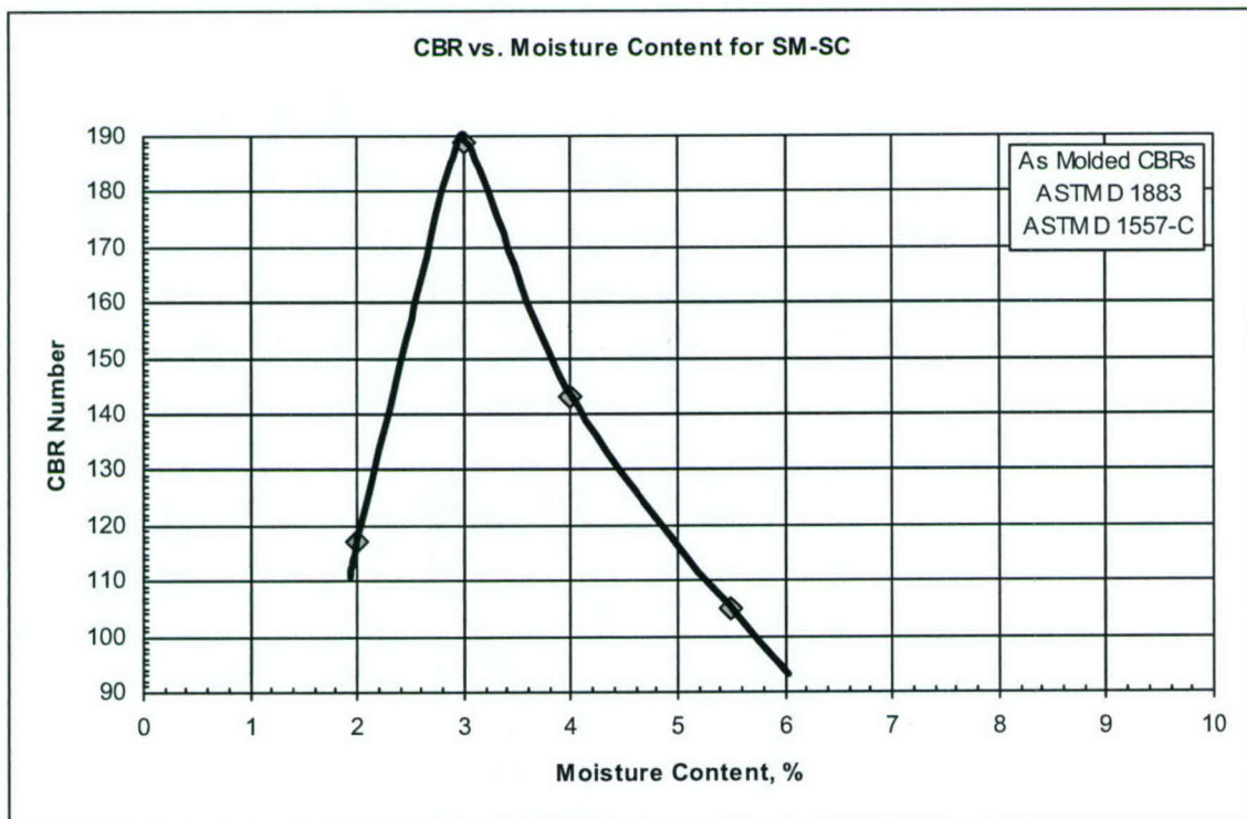
Figure 23. CBR versus moisture content curve for SM-SC
