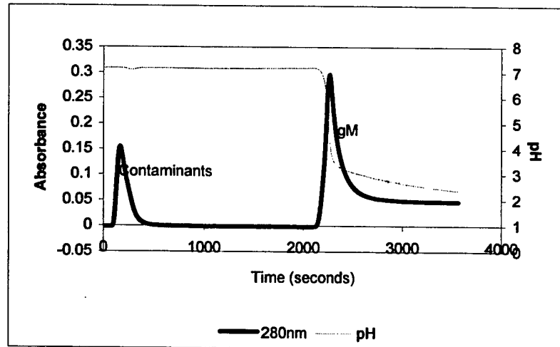
Figure 6. Chromatogram of IgM Antibody Purification Using an Anti-IgM Antibody Coupled Sepharose Affinity Chromatography Step.
