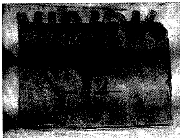
Figure 8. SDS-PAGE Results of the IgM In-process Samples. Lane #1: Molecular Weight Ladder, Lane #2: Sigma IgM Standard, Lane #3: Crude Cell Culture, Lane #4: Post GFC Purified IgM, Lane #5: Post Anti-IgM Column Purified IgM.
