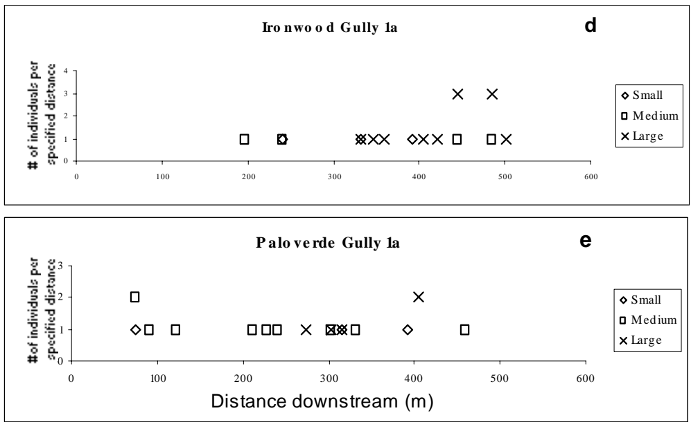
Fig. 12. Similar to data in Fig. 11, except for two arboreal species. Relative size (height) is indicated by the type of symbol. Species first appear tens to hundreds of meters downstream from gully tip. “Small”, “medium” and “large” designations defined in text.
