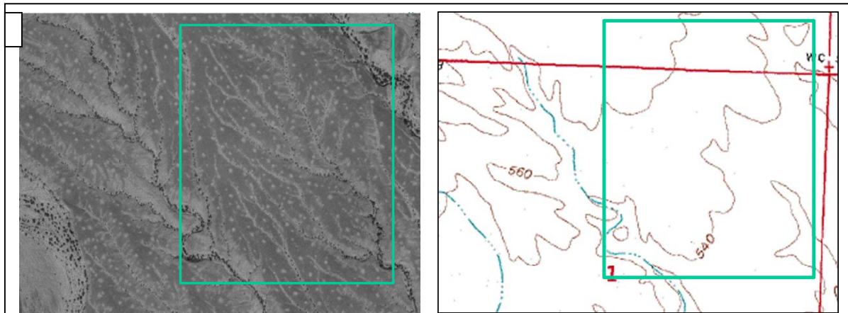
Fig. 2. (a) (left) Aerial photograph of study area (rectangle), short dimension of rectangle is about 1km; (b) (right) USGS topographic map of same area. Only the major drainage features are captured in the topographic map. The aim of ST is to combine the aerial photo map with the data from the low resolution map, using process based modeling, to produce a high resolution map that respects all the drainage ways shown in (a). The rectangle outlines the study area.
