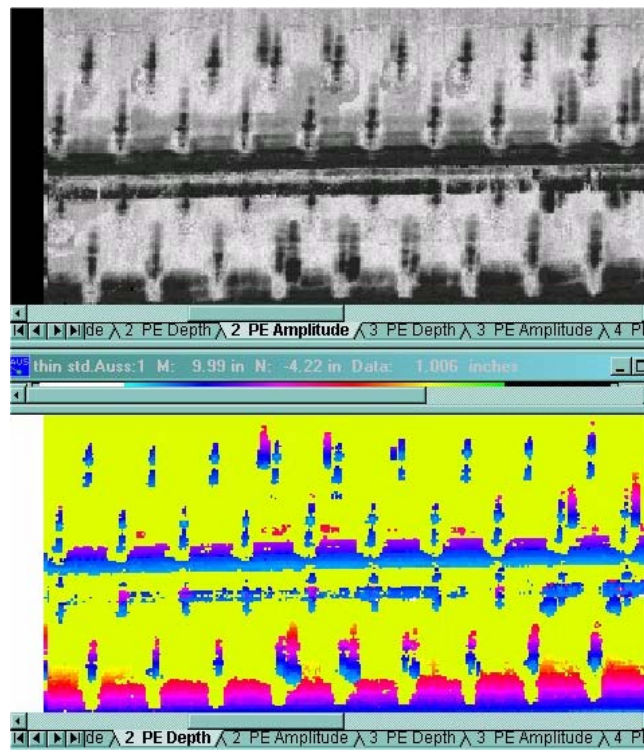
Figure 13: Pulse-echo C-scan data collected on B-52 reference standard showing spanwise flow locations (sensor 2 output)
