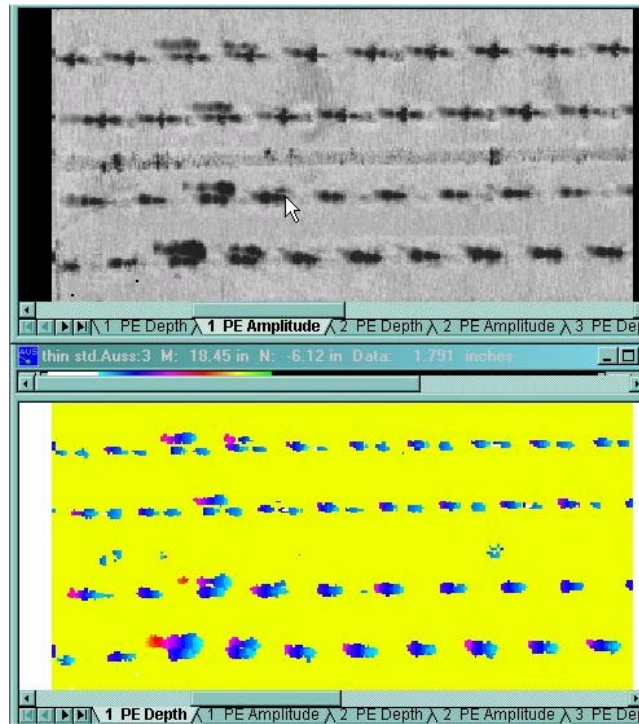
Figure 12: Pulse-echo C-scan data collected on B-52 reference standard showing chordwise flow locations (sensor 1 output)
