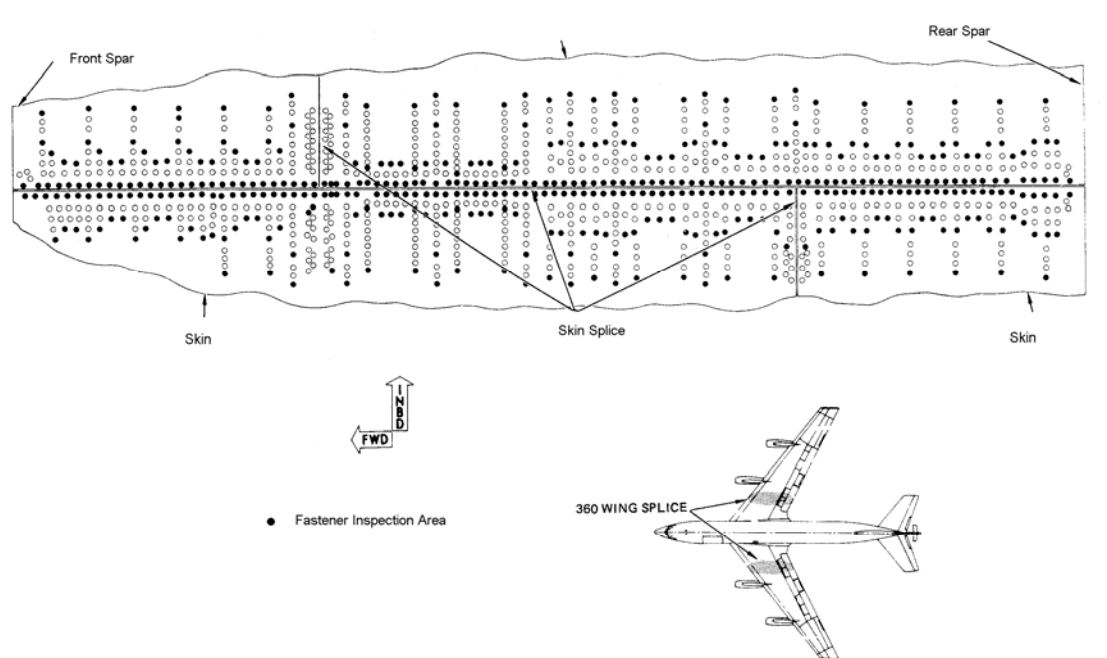
Figure 17: Sketch showing location of WS 360 splice on KC-135 wing.
