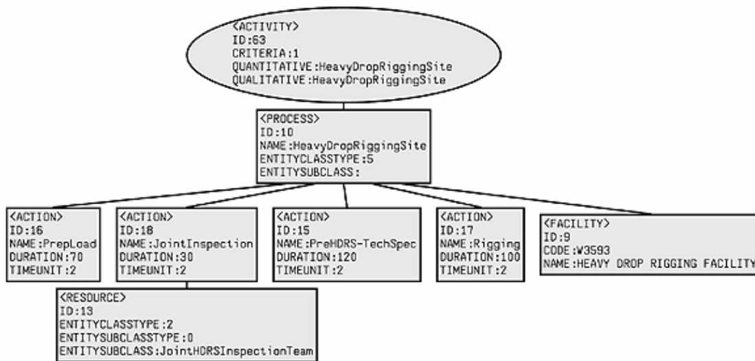
Figure 5. Sample output from Database Visualization Software.
