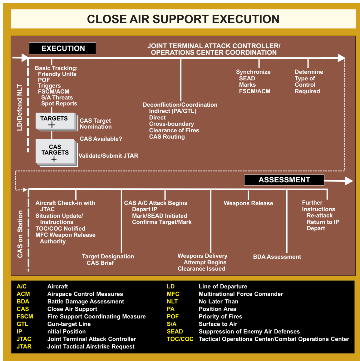
Figure V-1. Close Air Support Execution
