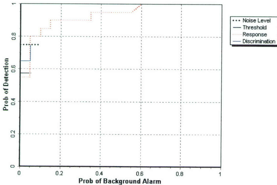
Figure 5. EM61 pushcart blind grid probability of detection for response and discrimination stages versus their respective probabilities of background alarm for all ordnance larger than 20 mm.
