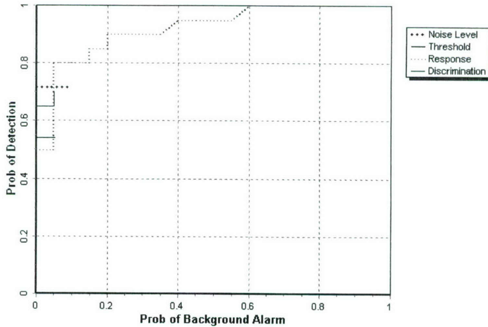
Figure 3. EM61 pushcart blind grid probability of detection for response and discrimination stages versus their respective probability of background alarm over all ordnance categories combined.
