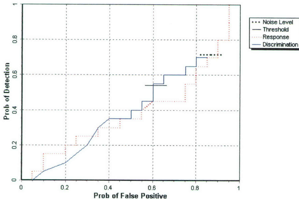
Figure 2. EM61 pushcart blind grid probability of detection for response and discrimination stages versus their respective probability of false positive over all ordnance categories combined.
