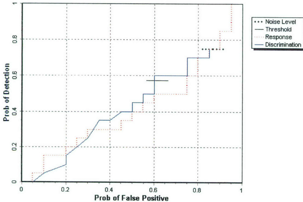
Figure 4. EM61 pushcart blind grid probability of detection for response and discrimination stages versus their respective probability of false positive for all ordnance larger than 20 mm.
