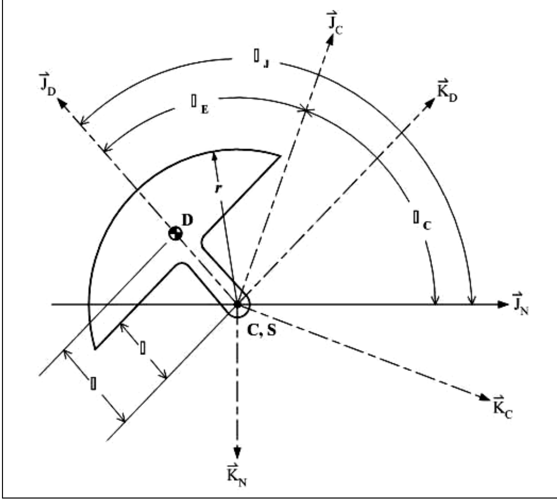
Figure 3. Internal part orientation angle control metrics.
