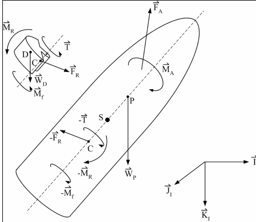
Figure 2. Free body diagram.
