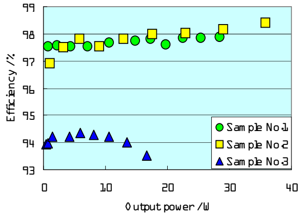
Figure 5. Efficiency vs. output power at the matching impedance of each sample.
