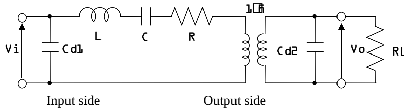
Figure 2. Equivalent circuit for a piezoelectric transformer.
