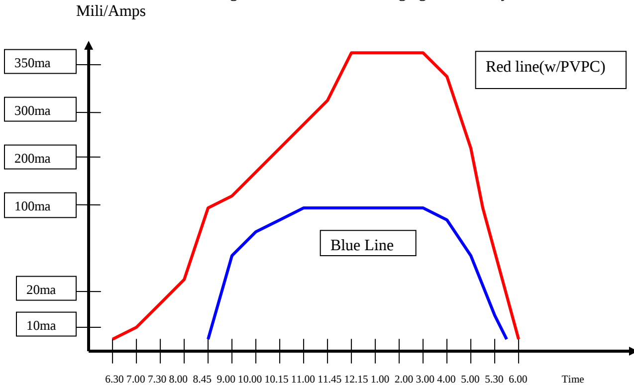
Figure 1. PVPC Test Recharging 12V Battery
