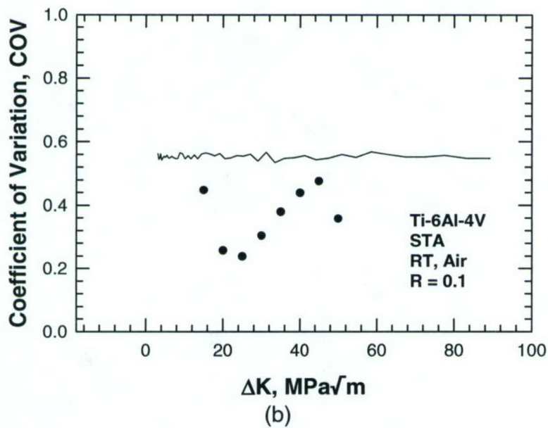
Figure 9. Comparison of computed crack growth rate predictions, probability density functions, and coefficient of variation (COV) with experimental data for R = 0.1 at 24^{\circ}\text{C} : (a) da/dN and probability density functions, and (b) coefficient of variation of da/dN .
