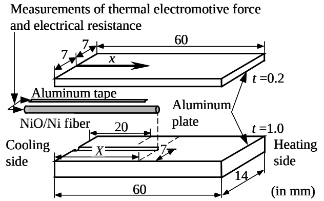
Fig. 10 Embedment of an insulated nickel fiber in aluminum matrix.
