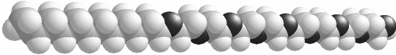
Octaethylene glycol monododecyl ether ( C_{12}EO_8 )
