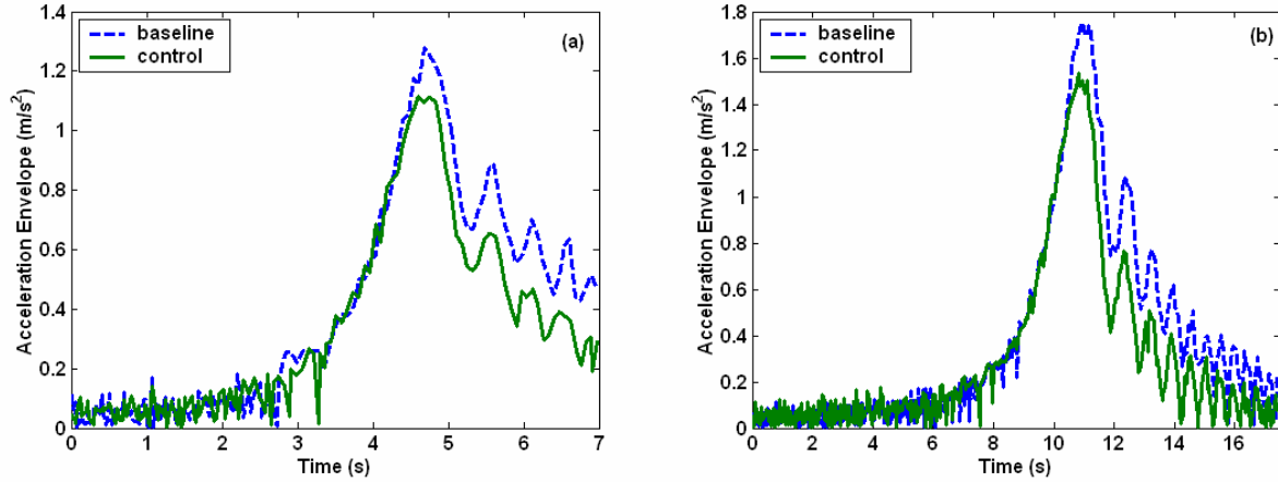
Figure 5 - Experimental acceleration envelopes for chirp excitation with rates of (a) 1 Hz/s and (b) 0.4 Hz/s
