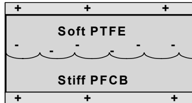
Figure 25 Schematic representation of a hybrid elastomer structure incorporating a porous PTFE and a stiff PFCB phase. 21
