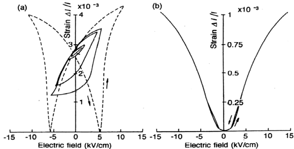
Figure 21 Electric field-induced strains in (a) piezoelectric lanthanum-doped lead zirconate titanate, and (b) electrostrictive lead magnesium niobate-based ceramics. 17
