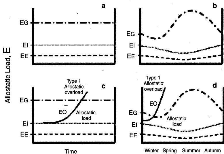
FIGURE 3-2 A framework for modeling energy requirements ( E ) of organisms during their life cycle. This energy requirement, E , includes all potential nutritional requirements, including energy itself. These separate and distinct requirements are represented more generally here for convenience, although essential components of nutrition could also be modeled separately. EE represents the energy required for basic homeostasis. EI represents the extra energy required for the organism to find, process, and assimilate food in ideal conditions. EG represents the amount of energy (in food) available in the environment (from Wingfield et al., 1998; Wingfield and Ramenofsky, 1999). (a) The three are represented as straight lines when environmental and physiological states do not vary over time. (b) The changes in the quantities have been adjusted to represent probable seasonal changes. EG would be expected to rise dramatically in spring and summer, when primary productivity is high, and then decline through autumn and winter, when primary productivity is low. In this scenario, EE would be lowest in summer, when ambient temperatures are highest. EI should be fairly constant (under ideal conditions) and should vary in parallel with EE . (c) EO represents additional costs incurred after a perturbation (such as a storm or anthropogenic disturbance) that increases costs above EE + EI . It represents the energy required to find food, process it, and assimilate nutrients in nonideal conditions. Allostatic load (see text) increases as EO persists. If EO exceeds EG , type 1 allostatic overload begins, resulting in an increase in plasma glucocorticosteroids. That usually triggers an emergency condition that results in altered physiology and behavior that reduces allostatic overload. (d) In more naturally fluctuating conditions, type 1 allostatic overload may occur first or more rapidly if a perturbation occurs during a season when the conditions are worse. If insults are permanent—such as those caused by even mild or moderate but persistent disturbances
