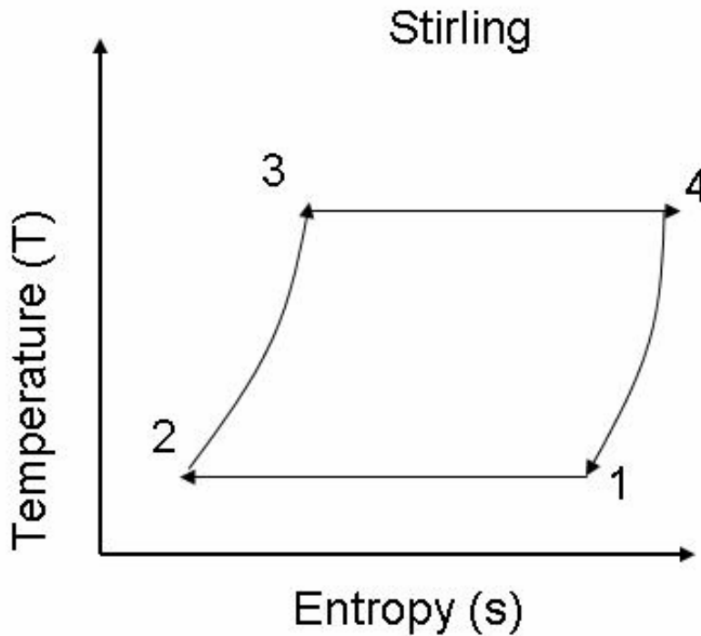
Figure 16. Ideal Stirling Temperature/Entropy Diagram
