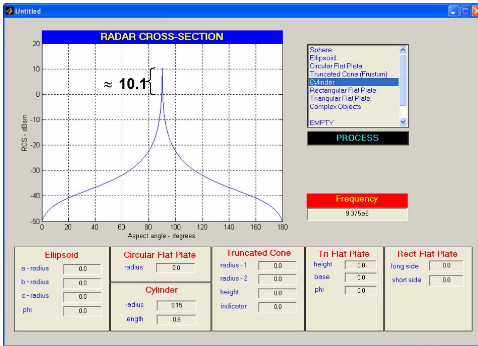
Figure 10. Graphical Representation of the RCS of Small Target
