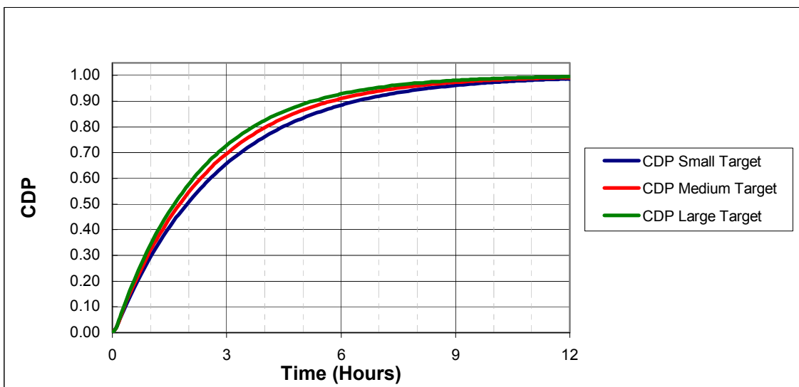
Figure 32. CDP vs. Time Applying 3,900 nm 2 and Nine-Hour Exposure
