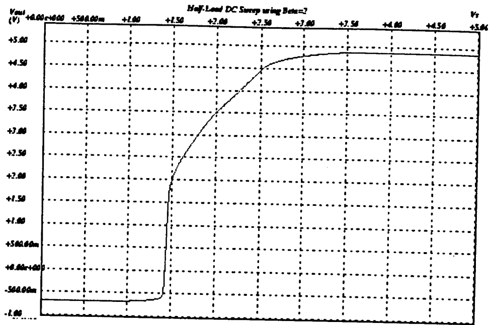
Figure 24: Half-load simulation with A_{V_{CL}} = 2 V/V from circuit in Figure 1.
