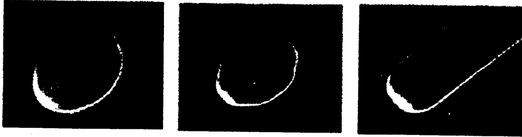
(a) (b) (c) Figure 1. RIE etched polyimide. Single layer (10 \mu\text{m} ). a) Circular, b) Octagonal and c) trench openings.
