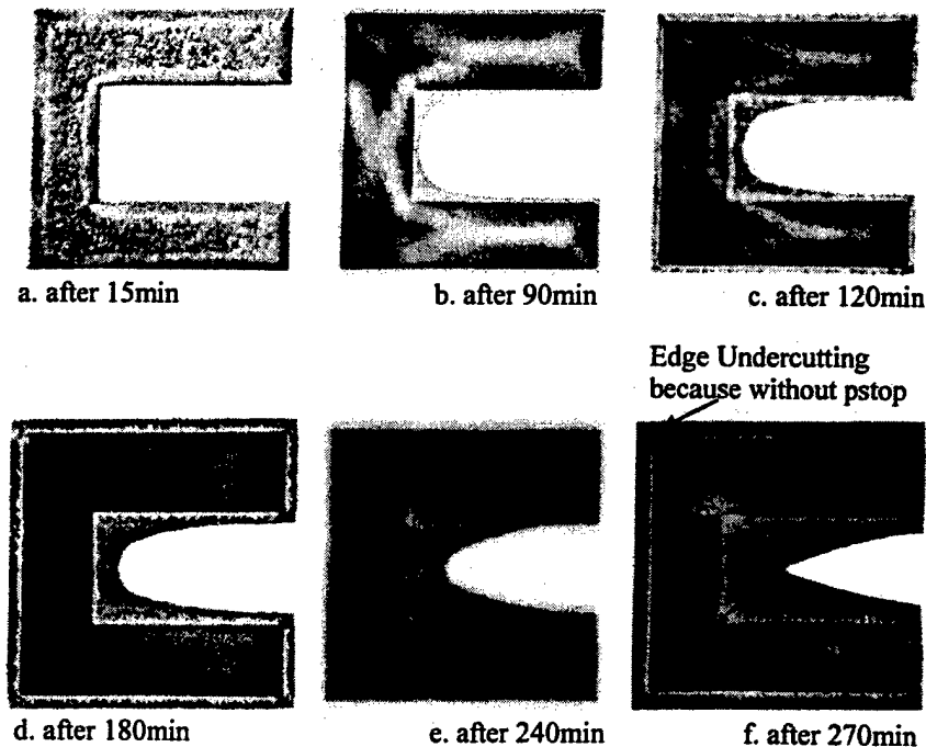
Fig.10 Undercutting evolving procedure (actual structure area size is 160μm x 160 μm)
