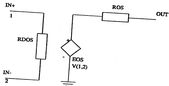
Figure 7: OUTSTG Stage
