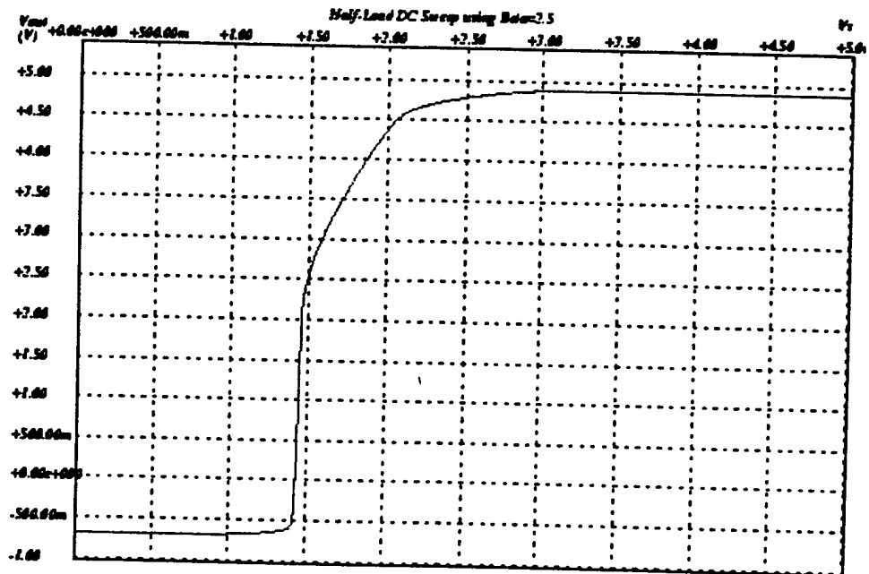
Figure 25: Half-load simulation with A_{V_{CL}} = 2.5 V/V from circuit in Figure 1.
