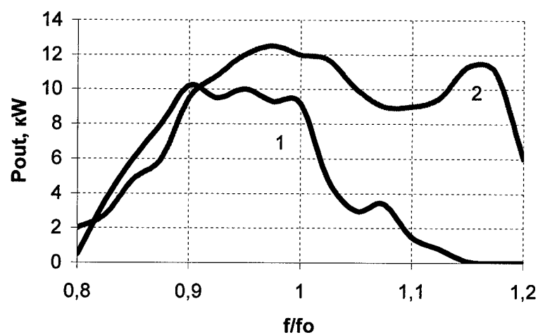
Fig. 6.7. Amplitude-frequency characteristics of the second model of plasma TWT
