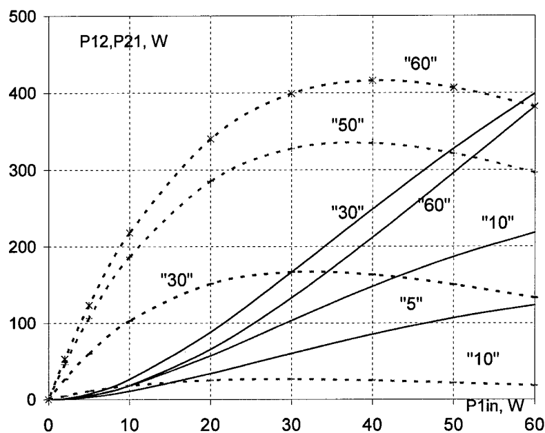
Fig. 7.5. The graphs of dependences of output power of combinational components of the third order P_{12out} (dotted lines) on input power level of the first signal P_{1in} at different fixed levels of P_{2in}
