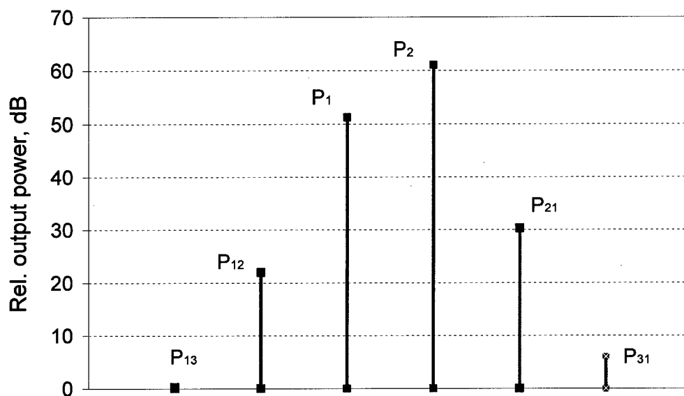
Fig. 7.3. Calculated spectrum diagram of output signal of plasma TWT at amplification of two input signals with P_{1\text{input}} = 5 \text{ W} , P_{2\text{input}} = 40 \text{ W}
