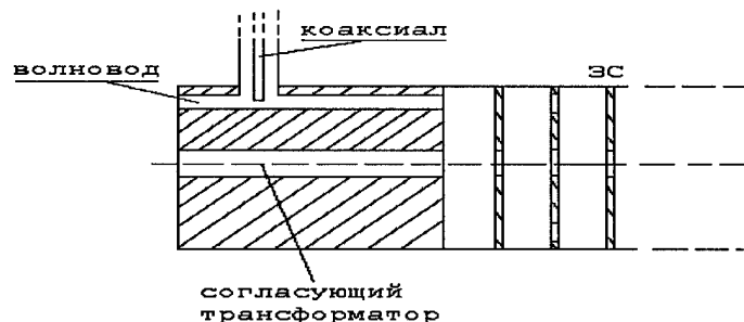
Fig. 4.2. The schematic view of matching transformer as the coaxial-wave guide adapter
