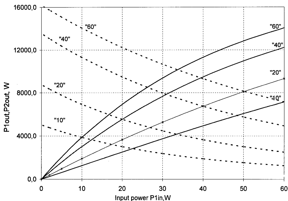
Fig. 7.4. The graph of dependences of basic signals output power P_{1\text{out}} (solid curves) and P_{2\text{out}} (dotted lines) on the first signal input power level P_{1\text{in}} at different fixed levels P_{2\text{int}} (values P_{2\text{int}} are designated in watts near the corresponding curves)
