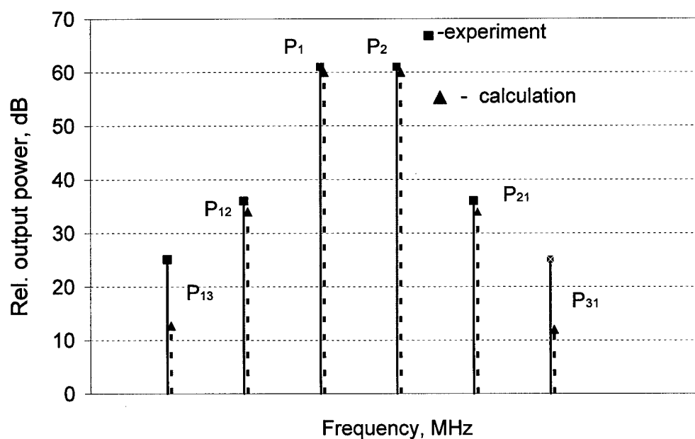
Fig.7.8. Experimental and calculated spectrum diagrams of output plasma TWT signal at amplification of two input signals, at P_{1in}=P_{2in}=20 \text{ W}
