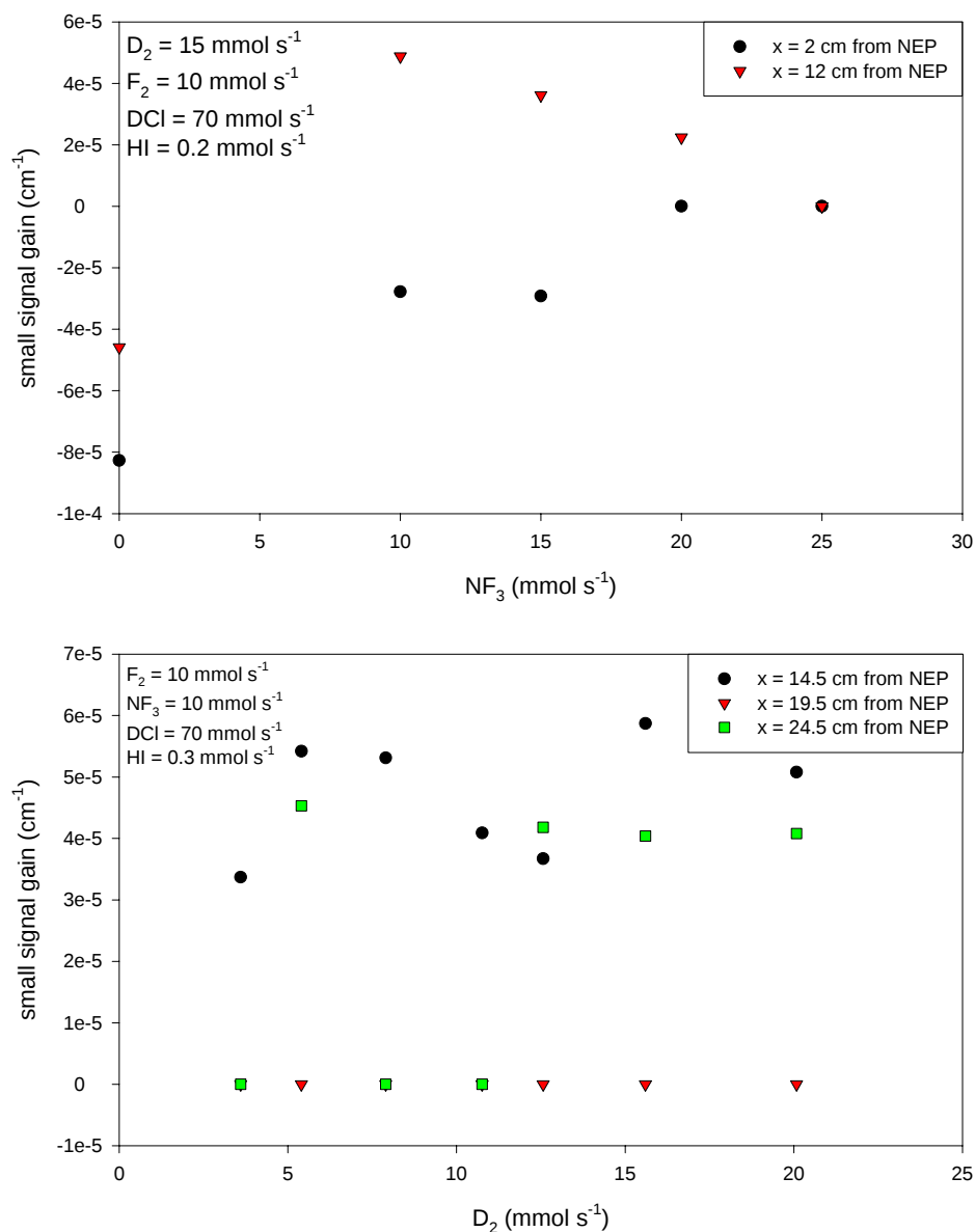
Figure 19. Small signal gain vs. \text{NF}_3 and \text{D}_2 .
