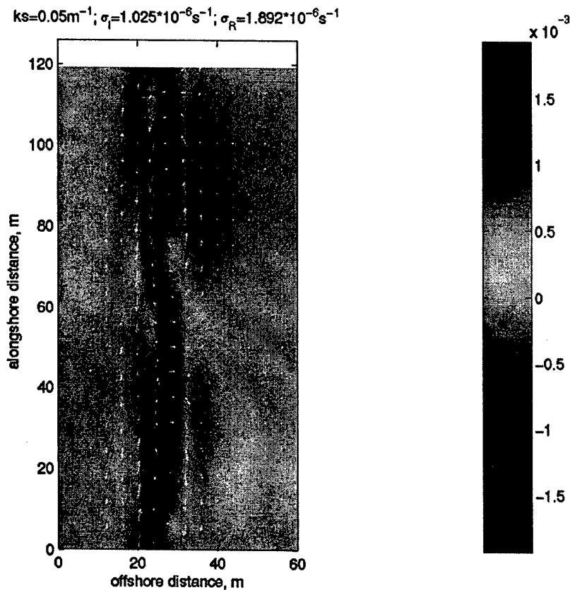
Figure 3: Spatial characteristic of the perturbation to an initially planar beach over an approximately 120m alongshore length scale. The outer edge of the surf zone is ~40m away from the shoreline. The circulation field is indicated by the arrows and is in the form of a rip current existing at the low point of the perturbation (the “hole”) and flow returning over the high point (the “hump”).
