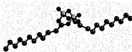
Figure 2. Molecular structure of \text{C}_{12}\text{H}_{46}\text{B}_2\text{O}_4\text{F}_3 . The carbon, oxygen, boron and fluorine atoms are shown in gray, red, green and blue, respectively. The hydrogen atoms are omitted.
