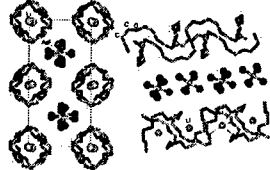
Fig. 1 Crystal structure of P(EO) 6 :LiAsF 6
