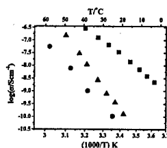
Fig. 3. Comparison of \sigma of P(EO) 6 :LiSbF 6 prepared from PEO M_w 1000 (squares), 1500 (triangles) and 2000 (circles)
