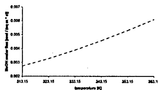
Figure 6. Methanol molar flux through the membrane as a function of temperature for Nafion™117 membrane, current density of 100 mA / sq cm, and membrane anode-side methanol concentration of 500 mol / cu m.
