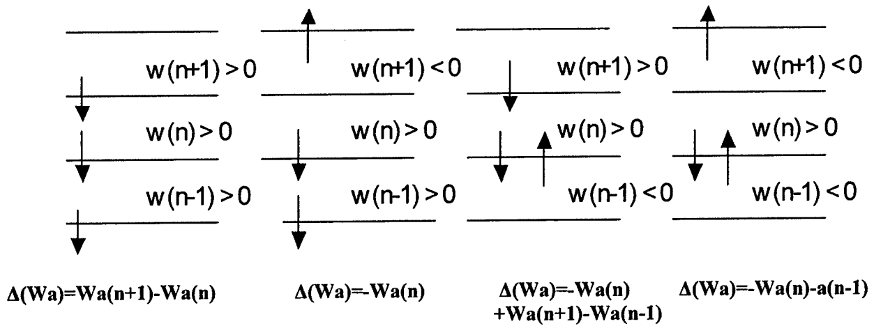
Figure 1. If w is the net vertical velocity including both gravitational settling and vertical air velocity and Wa is the air velocity, then the added air (velocity) consistent with the vertical motion of the particle in the given cell and section is given by \Delta(Wa) . For downward motion of the particle in cell n , \Delta(Wa) is the appropriate airflow into or out of the cell n for a given section, where positive flow is downward. There is a similar diagram when the flow in cell n is upward.
