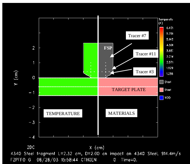
Figure 6. Simulation setup.
