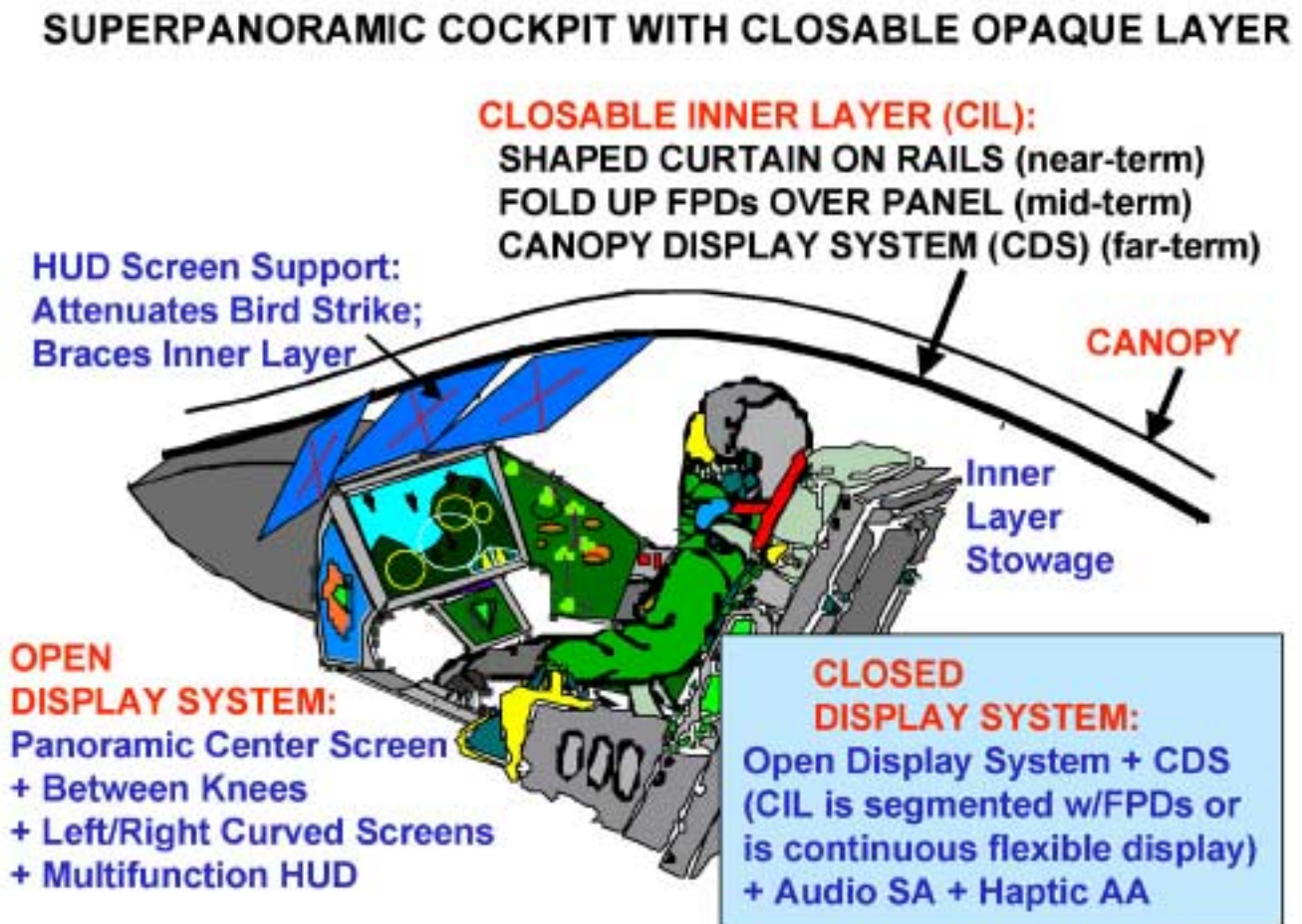
Figure 5. Concept for 2010: Super Panoramic Cockpit Plus
