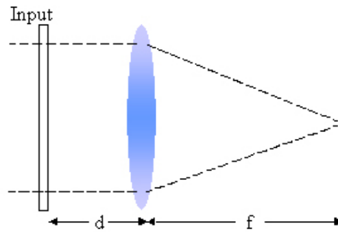
Figure 4.14: Positive lens as a Fourier transformer. 22
