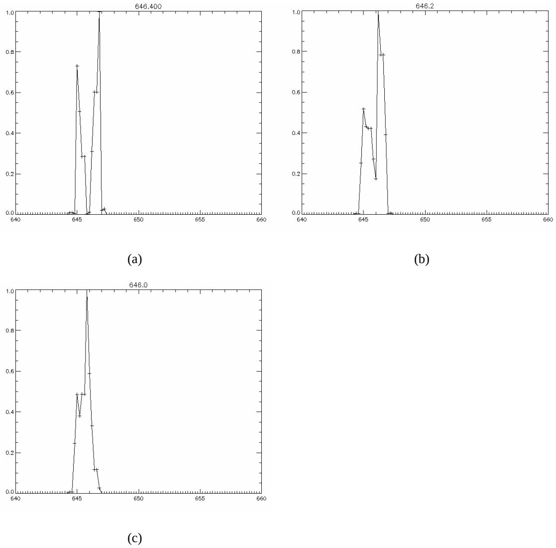
Figure B.2: Plots of the dual spectral components separated by (a) 1.4 nm, (b) 1.2 nm, and (c) 1 nm. Plot (b) is a repeat of Figure 5.9 and is the spectral resolution of the tunable CTIS according to the Rayleigh criterion after centroiding and upsampling but before convolving by the PSF.
