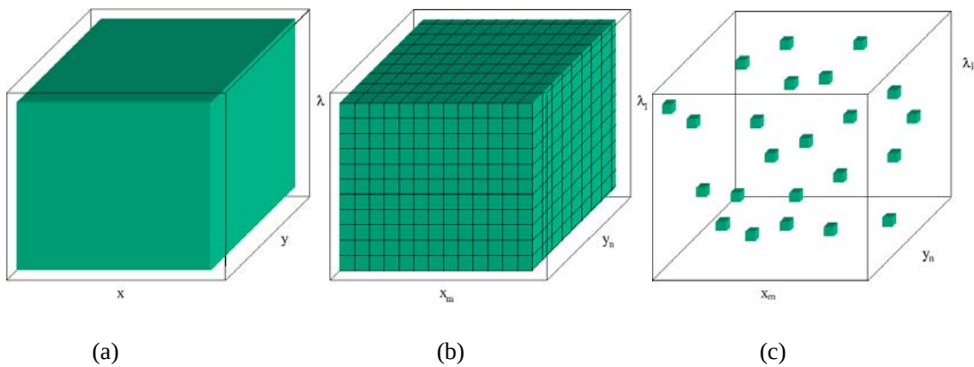
Figure 1.1: (a) The object cube, (b) discretized data cube, and (c) individual voxels of the data cube.
