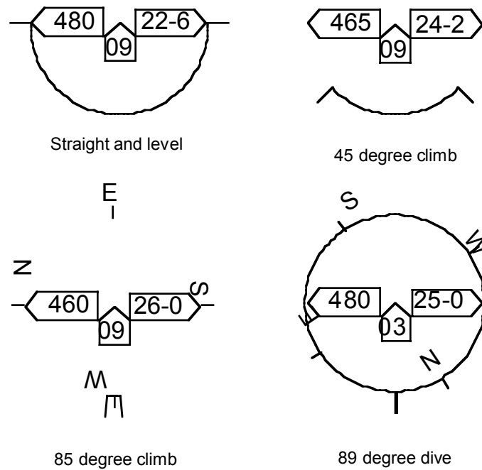
Figure 4. NDFR during various climb and dive angles.
