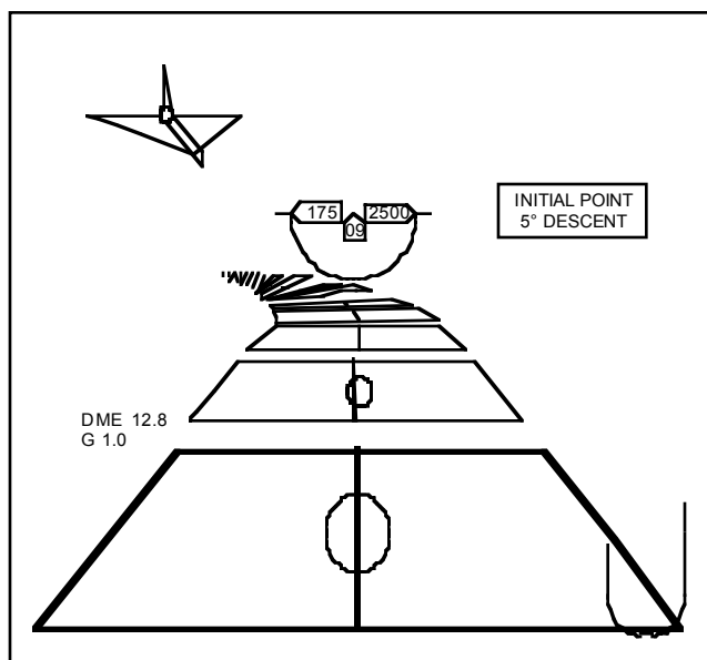
Figure 8. Flightpath-in-the-sky with NDFR ownship status information.
