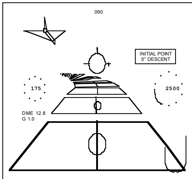
Figure 7. Flightpath-in-the-sky symbology with distributed ownship status information.
