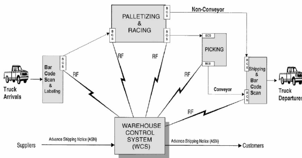
Figure 6.3.3: Typical logistical information flow with RFDC (Carlson, 1999)
