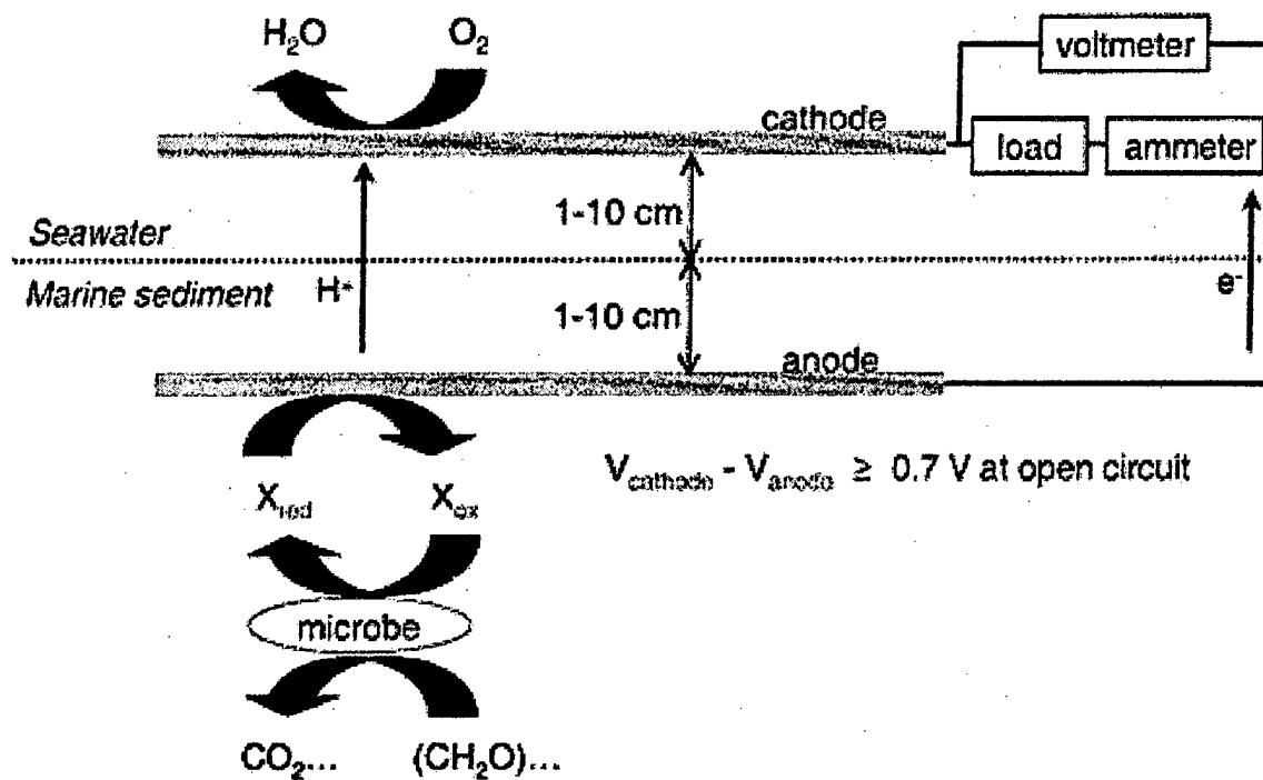
Figure 14. Schematic by Reimers et al. 20 illustrating the electrochemical processes of a microbially mediated battery.
