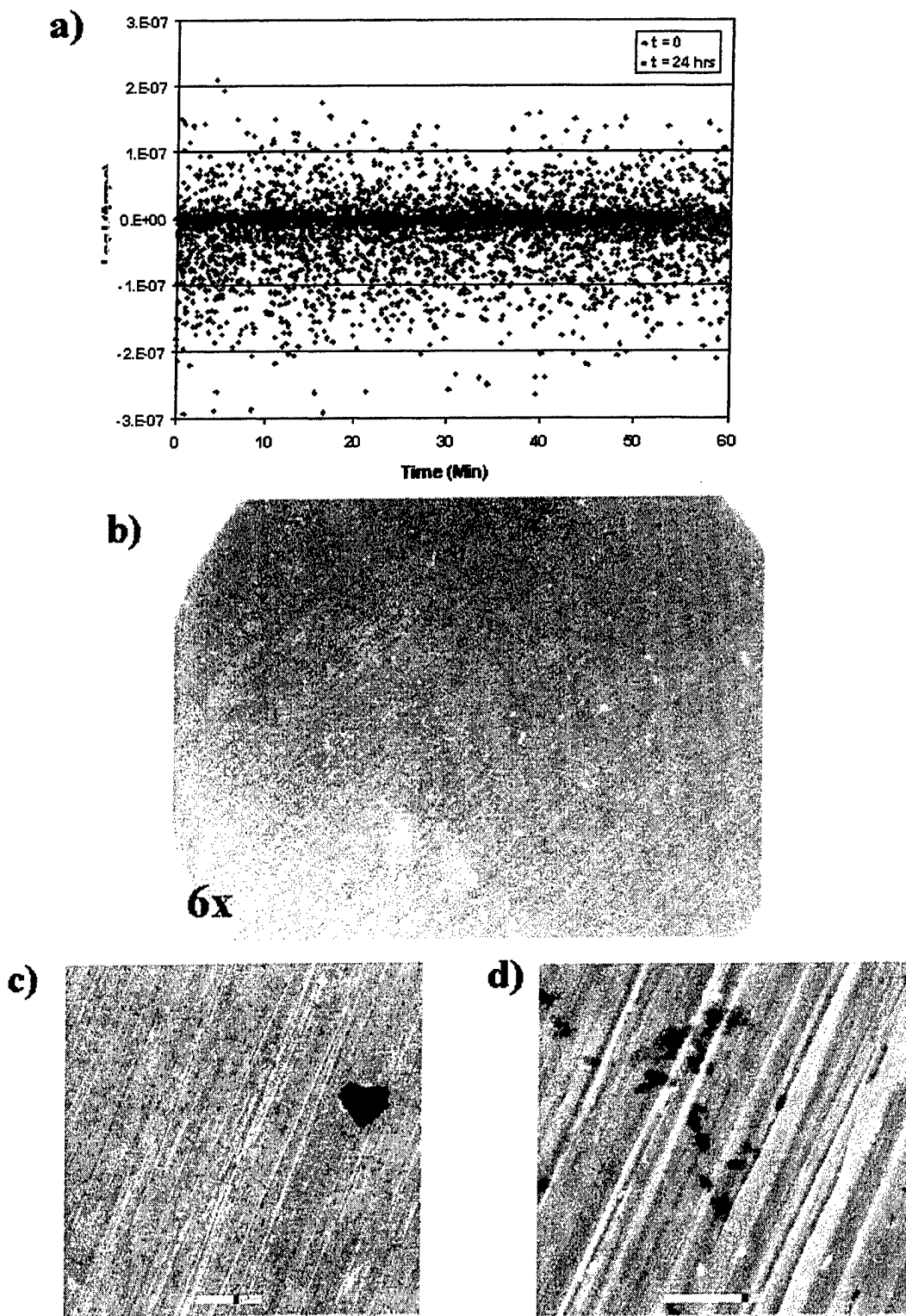
Figure 3. Laboratory electrode exposed to 1:100 Luria-Bertani in dH 2 O for 24 hrs with cathodic polarization. a) Applied current responses (linear scale) for potentiostatic holds (1 hr duration) at -175 mV vs. E_{corr} at exposure times of 0 and 24 hrs. b) Optical image of electrode surface after 24 hrs exposure. c&d) Micrographs of electrode surface after 24 hr exposure.
