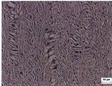
Figure 1: Optical micrograph of hot-rolled Ti-5111 plate showing coarse Widmanstatten alpha in a matrix of transformed beta. (micrograph taken from long transverse surface of plate)
