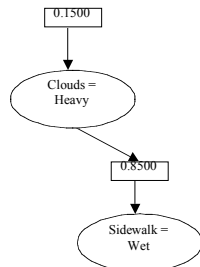
Figure 1. Example BKB.
