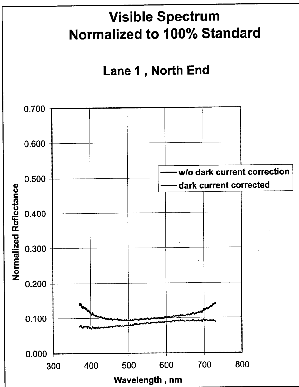
Figure 7-2. Visual reflectance spectrum of lane 1, North soil
