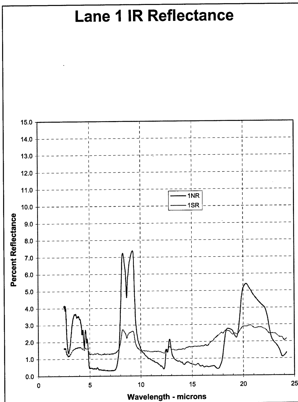
Figure 8-1. Broadband infrared reflectance, lane 1
