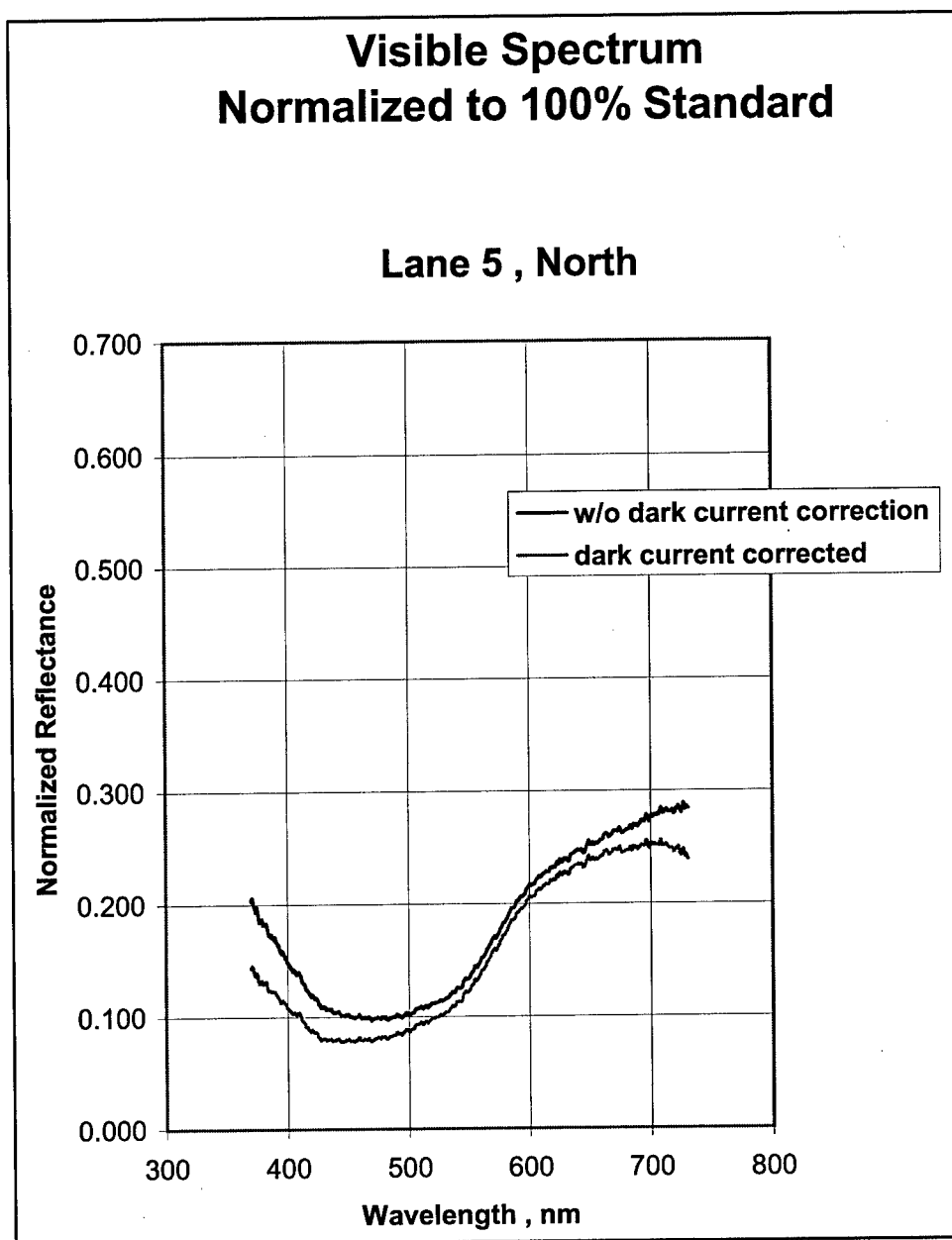
Figure 7-12. Visual reflectance spectrum of lane 5, North soil
