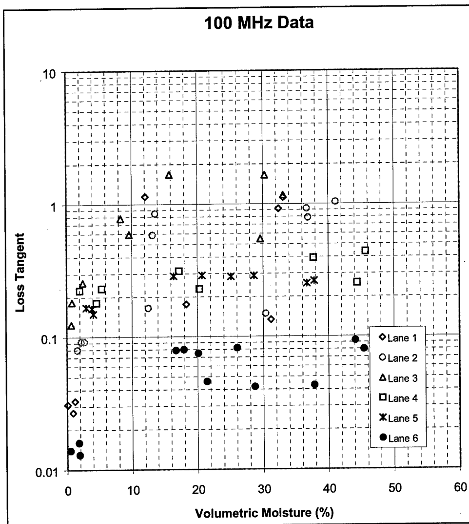
Figure 5-16. Loss tangent vs volumetric moisture, 100 MHz
