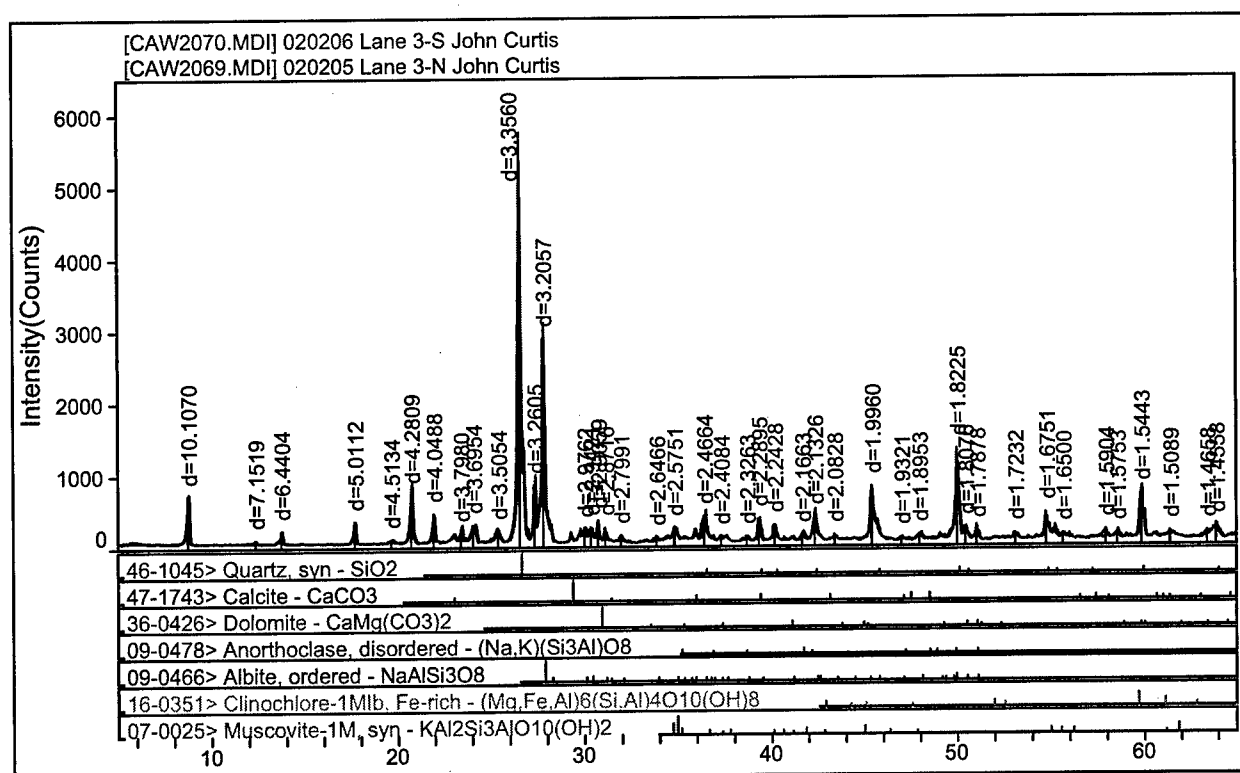
Figure 3-3. X-ray diffraction pattern of bulk samples of lanes 3N and 3S
