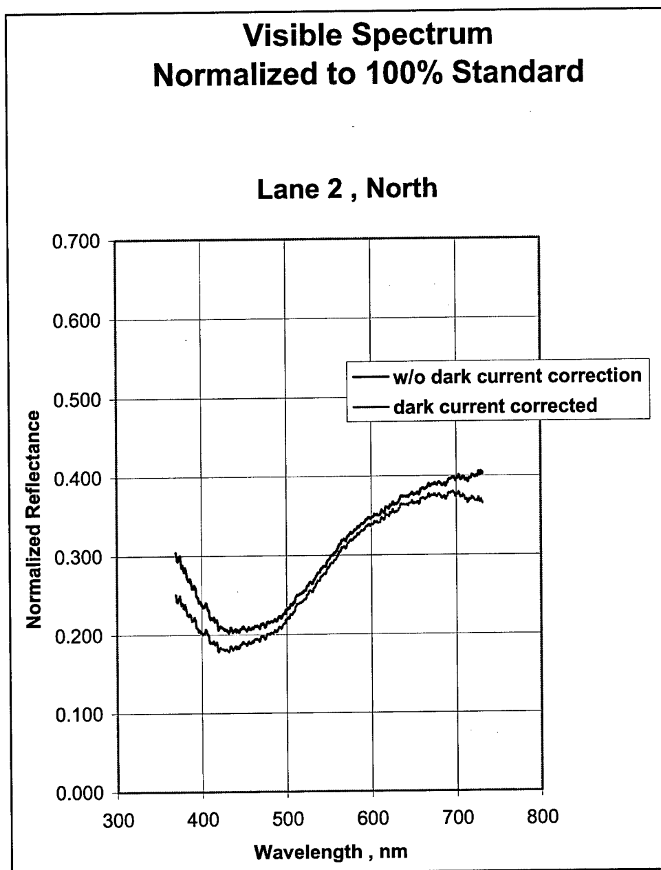
Figure 7-4. Visual reflectance spectrum of lane 2, North soil
