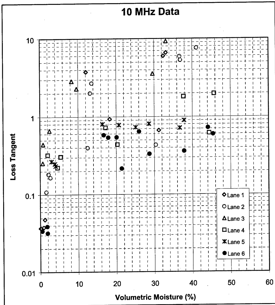
Figure 5-10. Loss tangent vs volumetric moisture, 10 MHz
