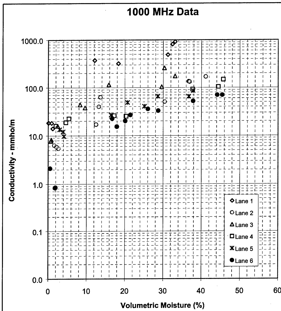
Figure 5-22. Conductivity vs volumetric moisture, 1,000 MHz
