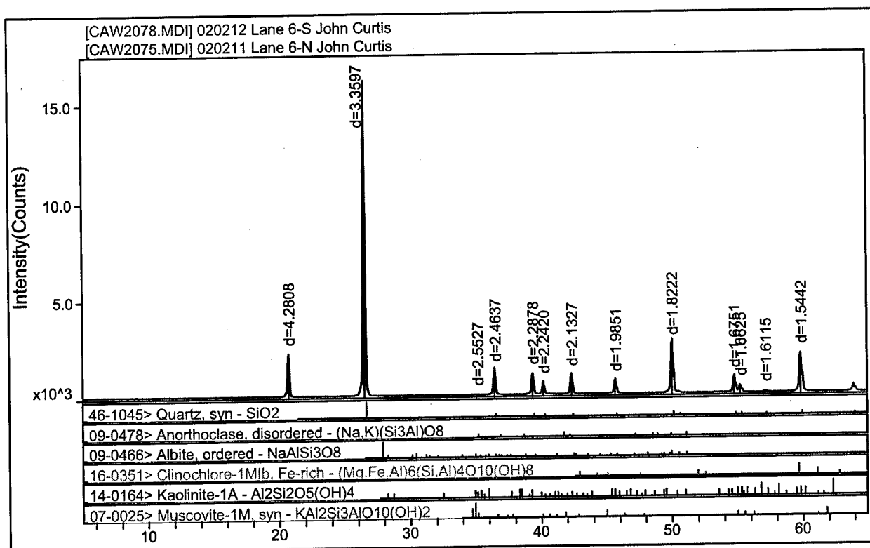
Figure 3-6. X-ray diffraction pattern of bulk samples of lanes 6N and 6S
