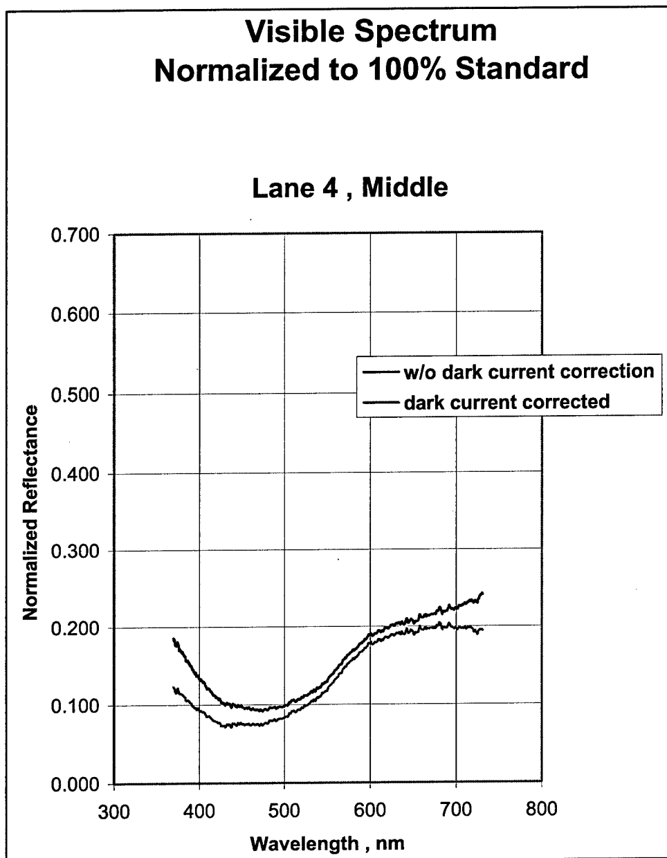
Figure 7-11. Visual reflectance spectrum of lane 4, Middle soil
