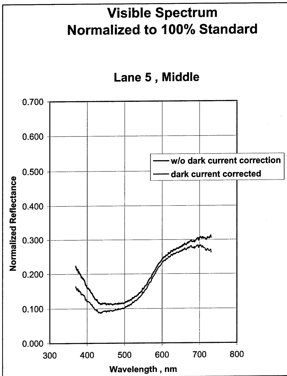
Figure 7-13. Visual reflectance spectrum of lane 5, Middle soil
