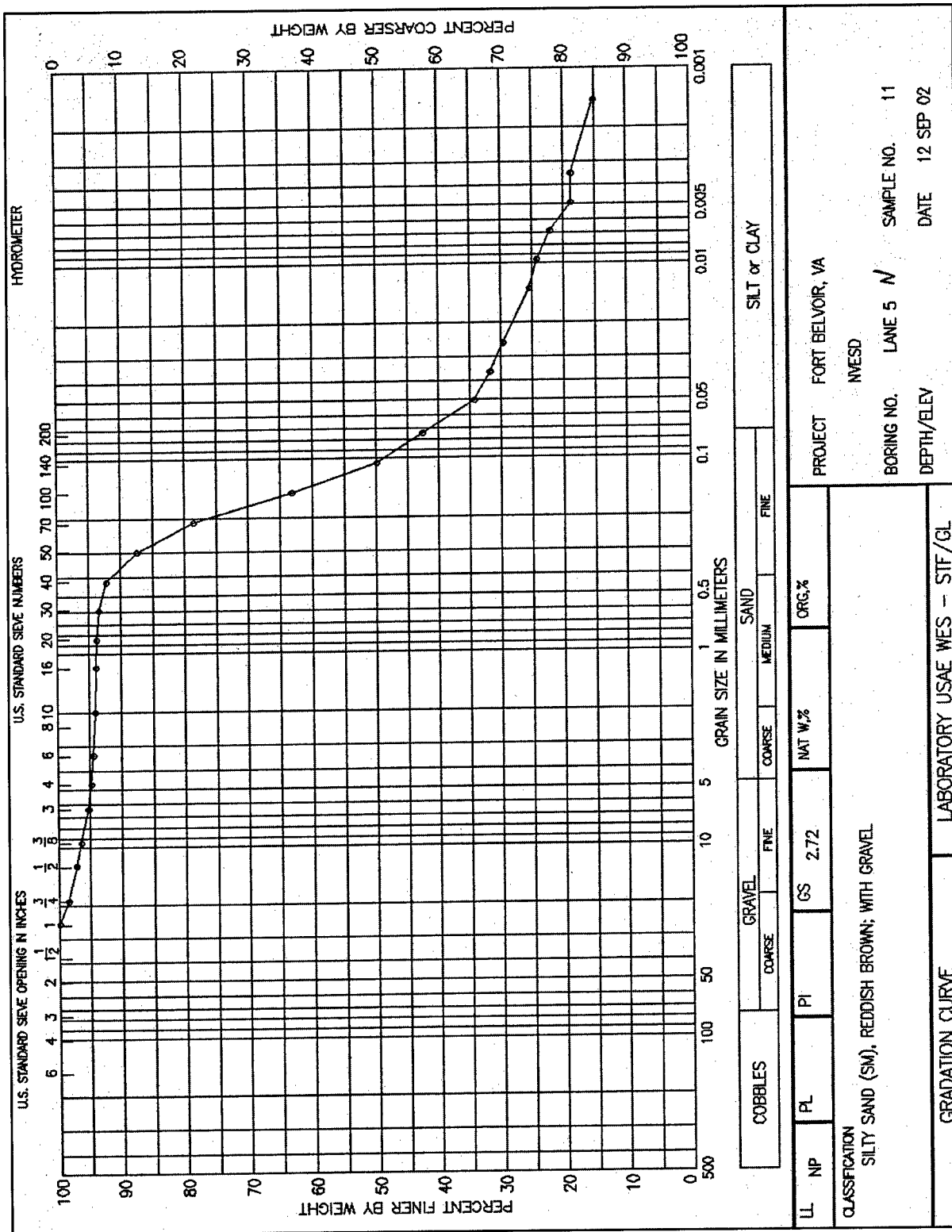
Figure 2-11. Gradation curve, Sample 11
