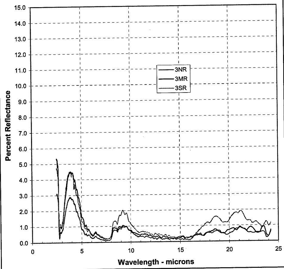
Figure 8-3. Broadband infrared reflectance, lane 3
