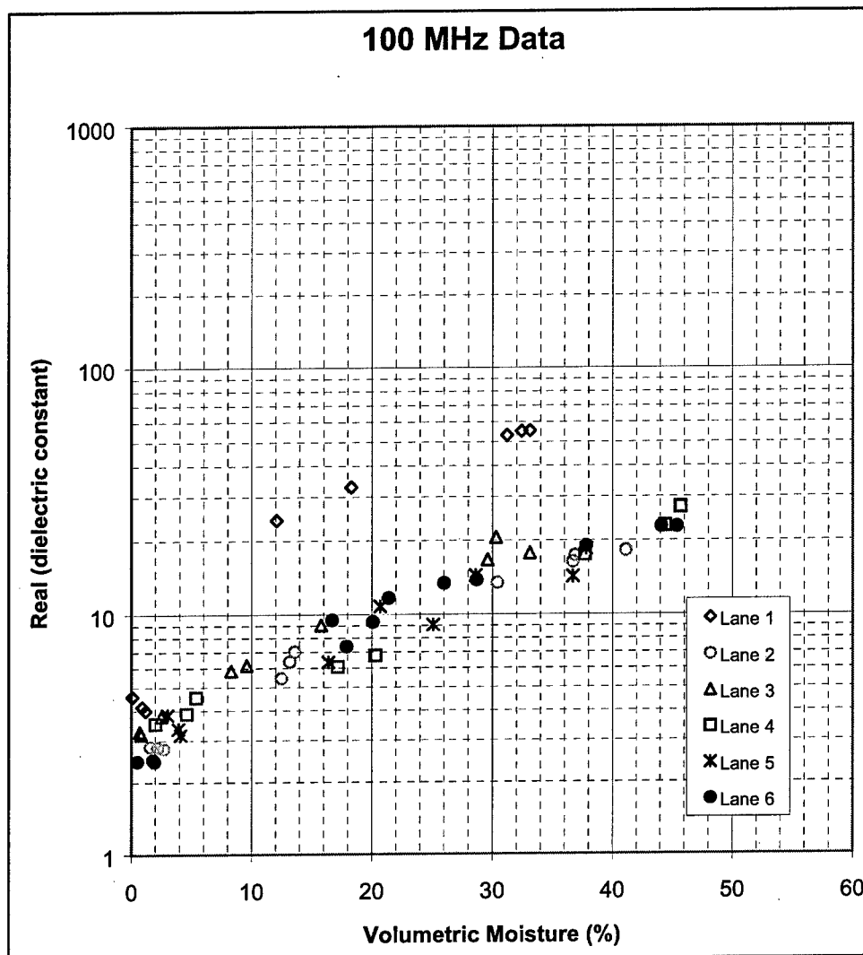
Figure 5-13. Real (dielectric constant) vs volumetric moisture, 100 MHz
