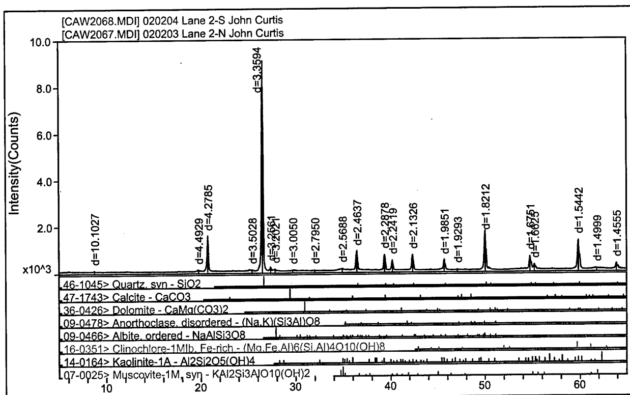
Figure 3-2. X-ray diffraction pattern of bulk samples of lanes 2N and 2S
