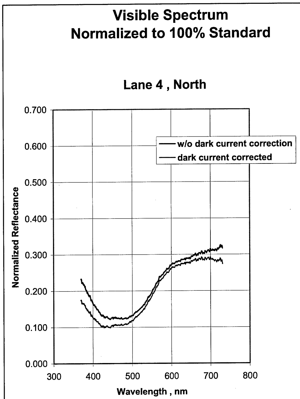
Figure 7-10. Visual reflectance spectrum of lane 4, North soil
