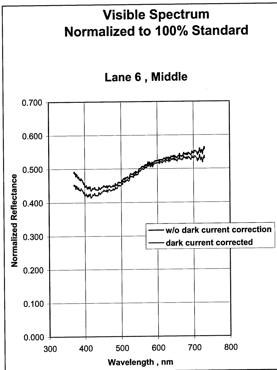
Figure 7-16. Visual reflectance spectrum of lane 6, Middle soil
