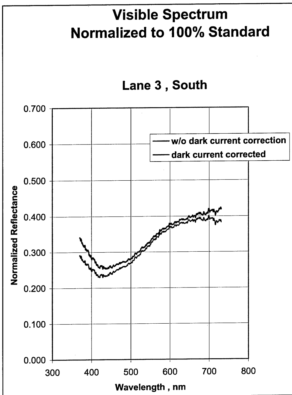
Figure 7-9. Visual reflectance spectrum of lane 3, South soil
