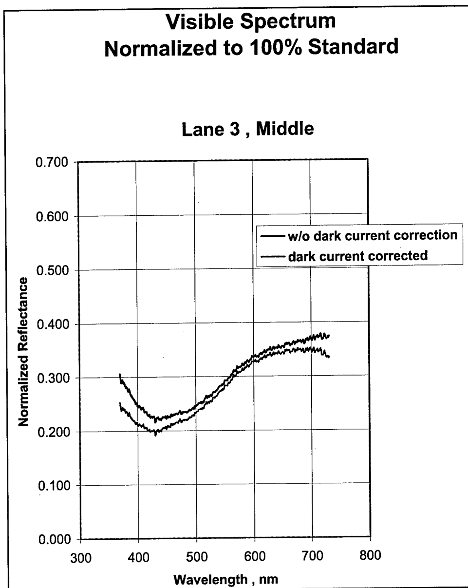
Figure 7-8. Visual reflectance spectrum of lane 3, Middle soil
