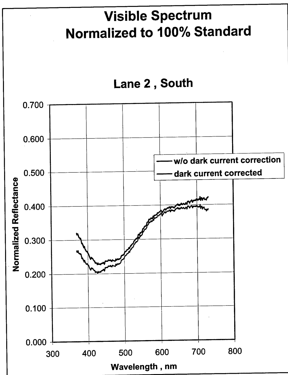
Figure 7-6. Visual reflectance spectrum of lane 2, South soil
