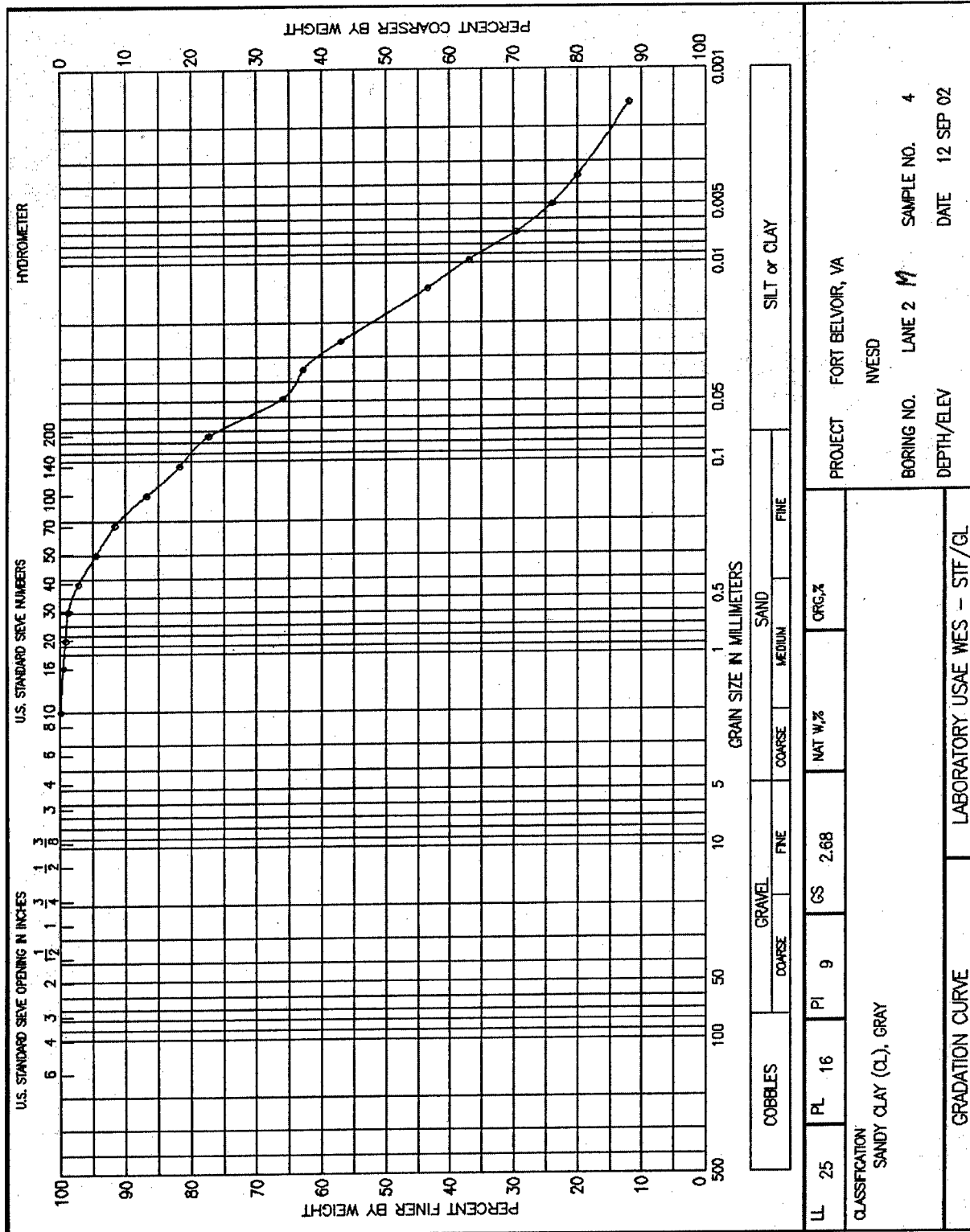
Figure 2-4. Gradation curve, Sample 4
