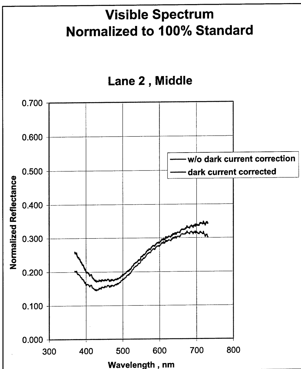
Figure 7-5. Visual reflectance spectrum of lane 2, Middle soil
