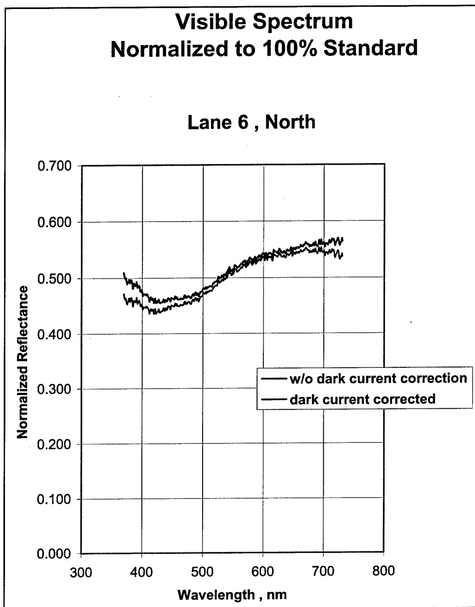
Figure 7-15. Visual reflectance spectrum of lane 6, North soil
