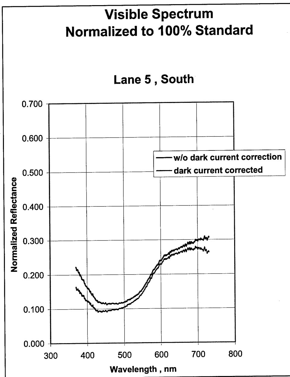
Figure 7-14. Visual reflectance spectrum of lane 5, South soil
