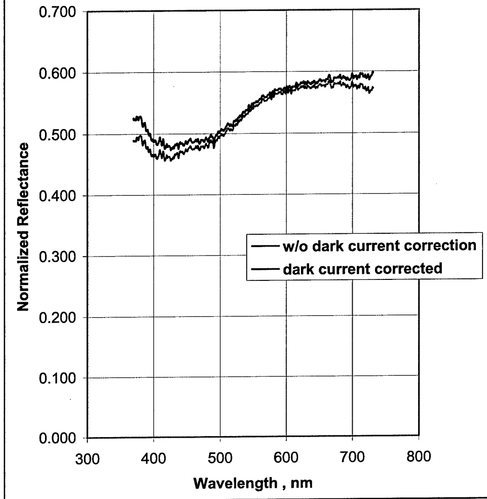
Figure 7-17. Visual reflectance spectrum of lane 6, South soil
