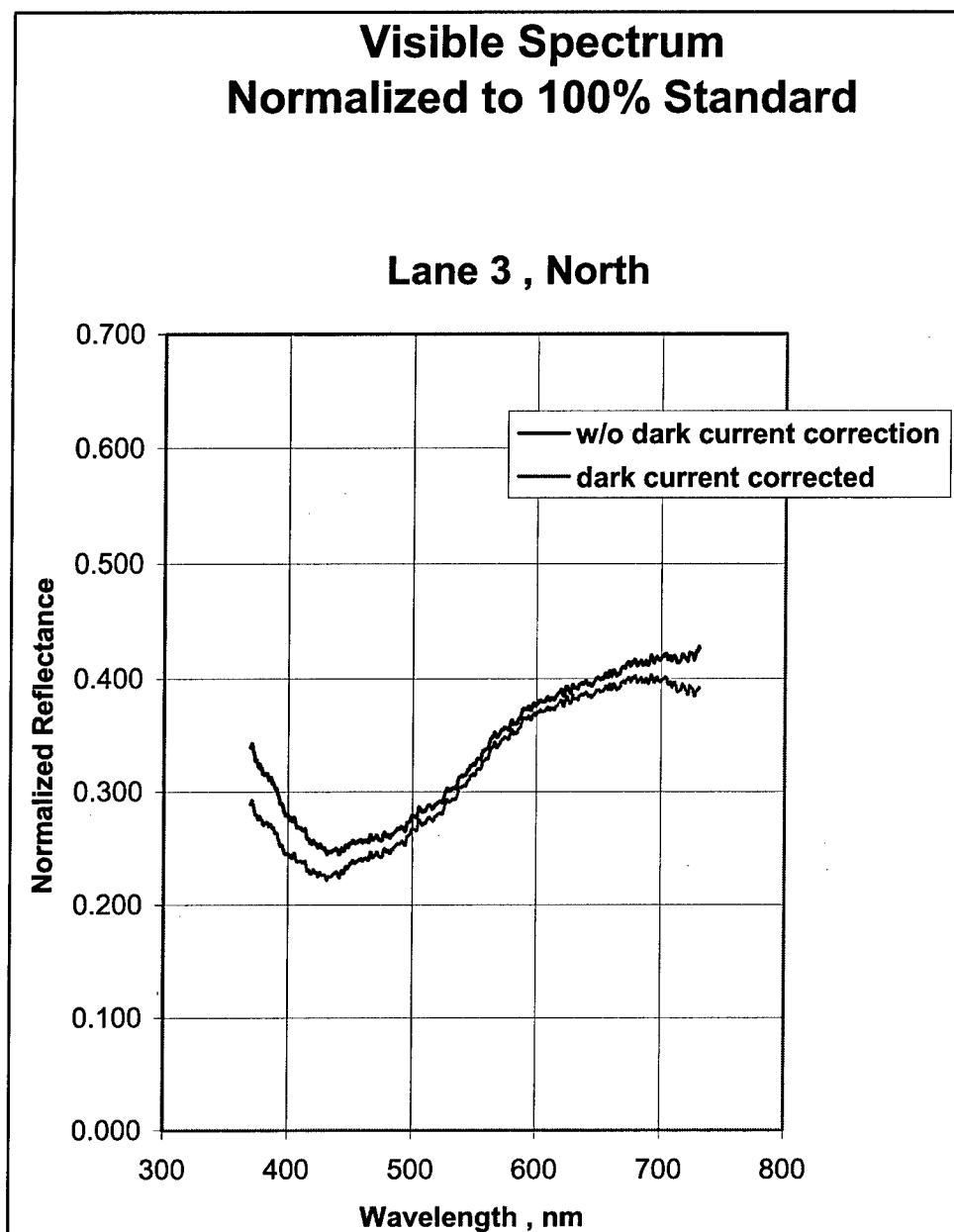
Figure 7-7. Visual reflectance spectrum of lane 3, North soil
