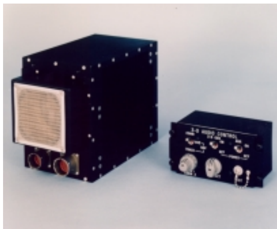
Figure 1. The Air Force Research Laboratory's 3-Dimensional Auditory Generator was used to generate virtual auditory cues that appeared to emanate from various locations along the horizontal plane.
