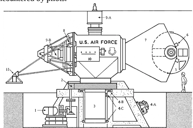
Figure 3. The Air Force Research Laboratory's Dynamic Environment Simulator centrifuge. (1) main arm drive motor; (2) drive pinion; (3) main rotating trunion and bull gear; (4a) hydraulic pumps; 4(b) thrust pad; (4c) upper and lower radial pads; (5) cab; (6) cab drive motor; (7) fork; (8) fork drive motor; (9a) main arm slip rings; (9b) fork slip rings; (10) motor driven counterweight; (11) aft-mounted platform.
