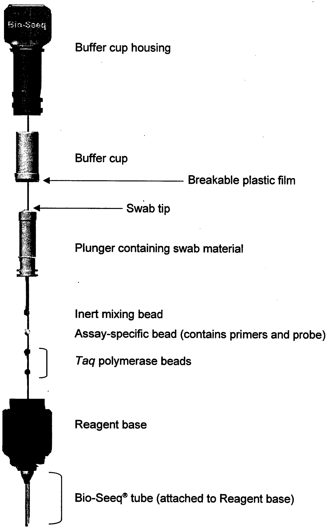
Figure 2. Consumable Sampling Device with Reaction Tube for the Bio-Seeq®
