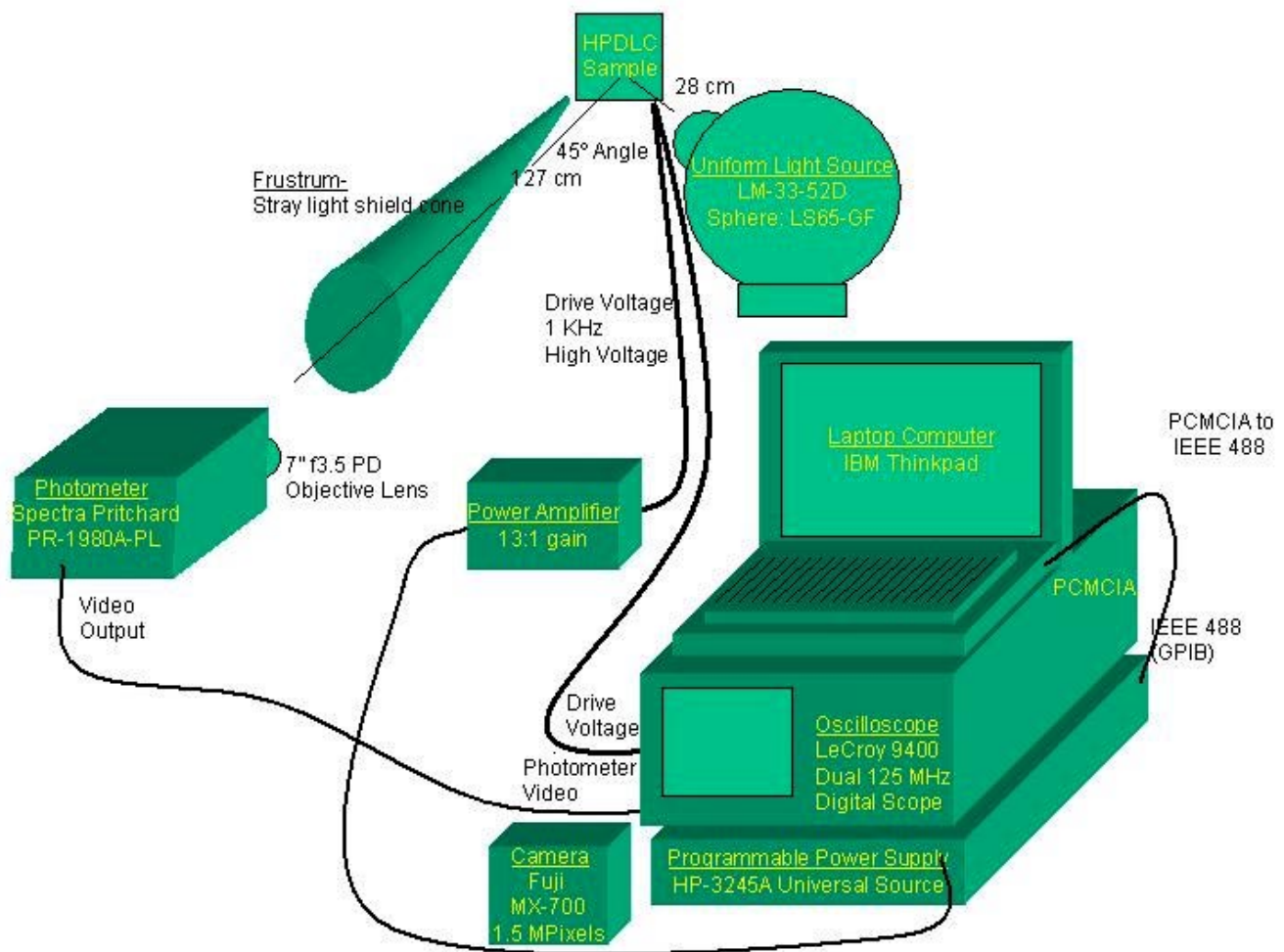
Figure 2. Laboratory test configuration
