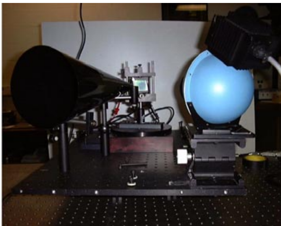
Figure 4. Front view of sample and frustum- rear view of light source
