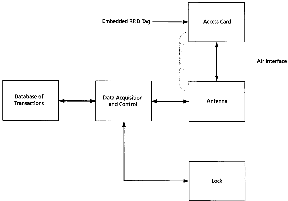
Figure 1 Elements of a Typical RFID Access Control System
