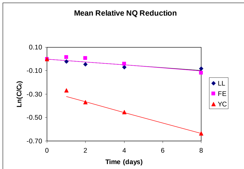
Figure 3. Logarithmic analyte loss with respect to time. Each data point is the mean of three sample measurements. The LL and FE trendlines, overlying one another, are least-square linear fits with zero y-intercepts.
