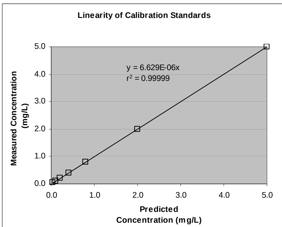
Figure 1. Calibration standards linearity. The trend line through the data is the least-squares best fit.
