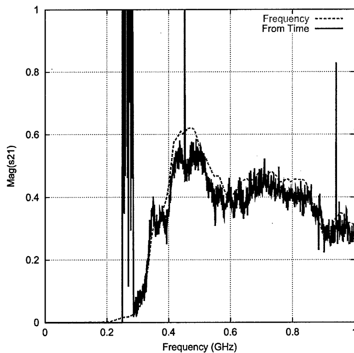
Figure 14: Magnitude of the measured transfer characteristic of a pair of horn antennas spaced 10" apart. The dashed line is a direct frequency measurement of the transfer function (s21), and the solid line is derived from the ratio of the Fourier transforms of the time-domain chirp waveform data.
