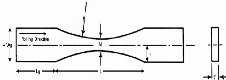
Figure 1: E466 tensile test specimen with continuous radius between ends geometry
