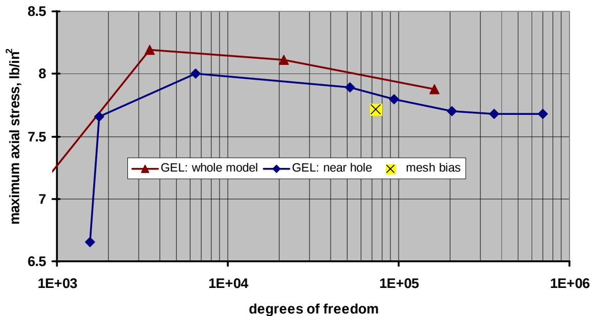
Figure 12: Degrees of freedom versus maximum net section stress for ASTM E466 specimen with 7/16 in net section through thickness hole
