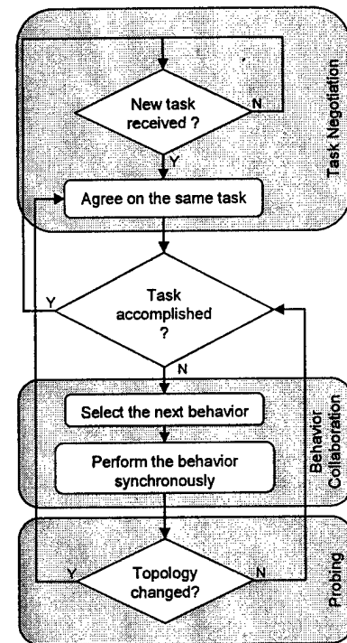
Figure 6: The FEATURE algorithm
