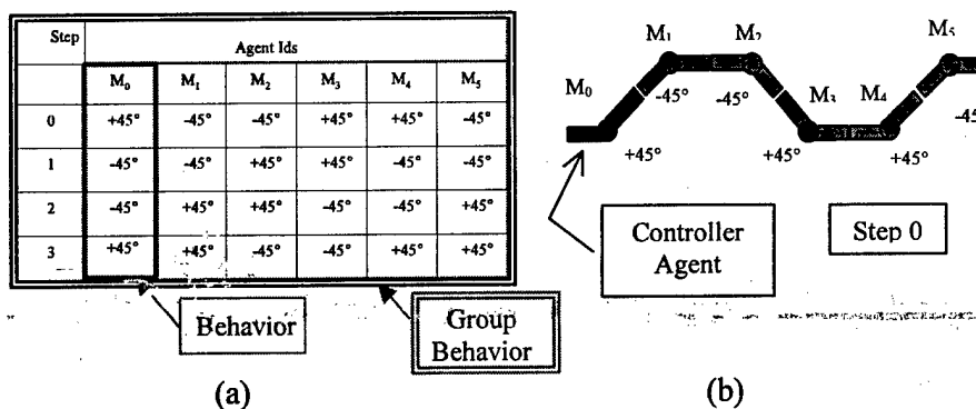
Figure 10: a) A central 'gait control table' controller for a caterpillar shape robot. b) A caterpillar robot performing step 0. Controller agent is the left-most agent, M 0
