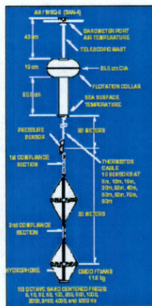
Figure 3: AN/WSQ-6 Specifications
