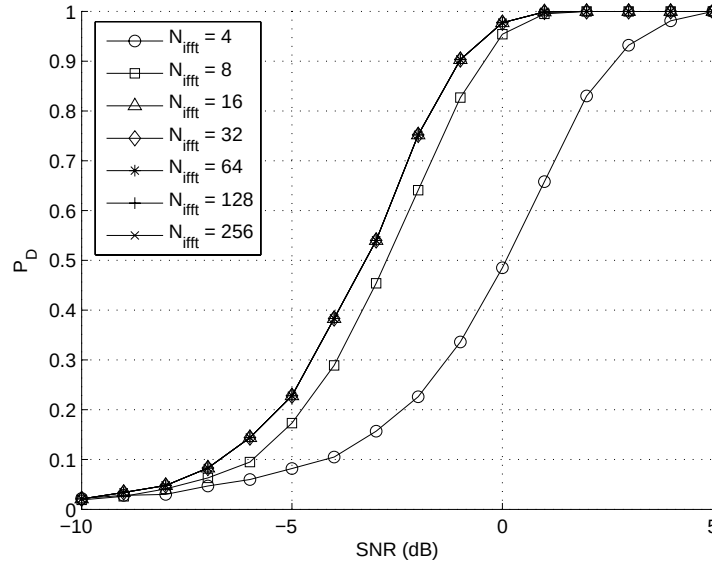
Figure A.21 CTM - 500 MHz DC ChRx (Varying Number of Points in IFFT)
