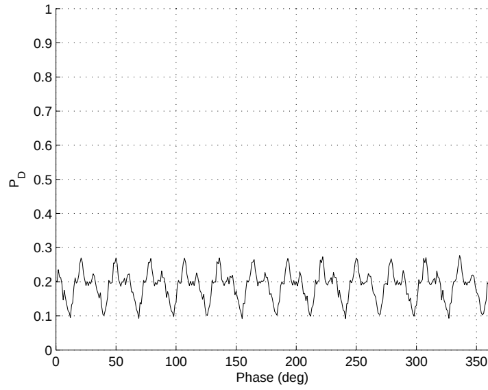
Figure A.28 SSM - 500 MHz DC ChRx, SNR = 0 dB (Varying Starting Phases)
