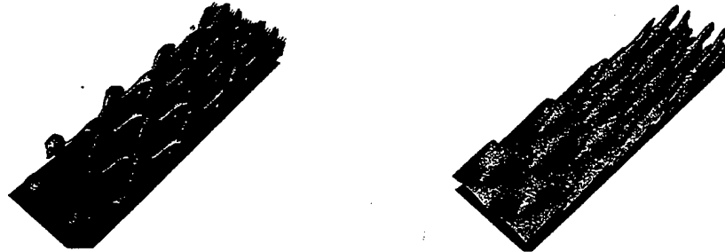
Figure 6.26 Isosurface of Q-criterion Q = 0.2 (left) and spanwise vorticity \omega_z = 15 (right) for a oblique fundamental resonance; Re = 10^5 , R_x = 705 - 925 , F = 5 \times 10^{-5} , \Psi_{1,1} = 60^\circ .
