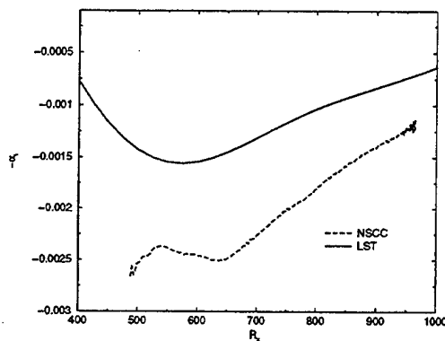
Figure 6.11 Amplification rate comparison of computations with results from LST for F = 5 \times 10^{-5} ( f^* = 10, 500\text{Hz} ).
