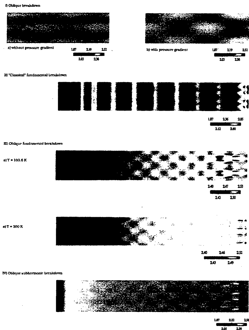
Figure 6.53 Near-wall temperature distribution for different breakdown scenarios. I) Oblique breakdown, F = 3 \times 10^{-5} , T_{\infty} = 103.6\text{K} . a) without pressure gradient. b) with pressure gradient. II) "Classical" fundamental breakdown, 1 st mode, F = 5 \times 10^{-5} , T_{\infty} = 103.6\text{K} . III) Oblique fundamental breakdown, F = 2 \times 10^{-5} . a) T_{\infty} = 103.6\text{K} . b) T_{\infty} = 300\text{K} . IV) Oblique subharmonic breakdown, F_{2,1} = 5 \times 10^{-5} , F_{1,2} = 2.5 \times 10^{-5} , T_{\infty} = 103.6\text{K} .
