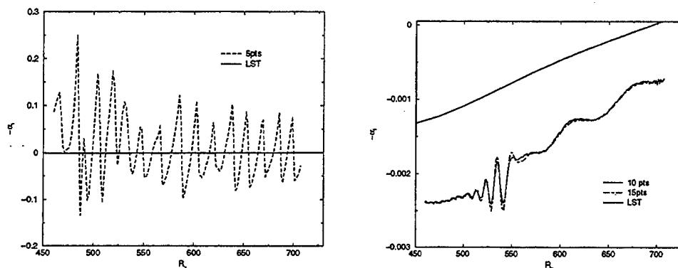
Figure B.7 Low resolution case (left) and higher resolution cases (right) in the y-direction (32 points per \lambda_x , 6\delta high).
