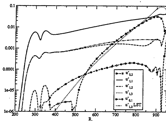
Figure 6.25 Oblique fundamental resonance: Amplitude distribution of u -perturbation versus downstream direction. Re = 10^5 , F = 5 \times 10^{-5} , \Psi_{1,1} = 60^\circ , \Psi_{1,2} = 74^\circ .
