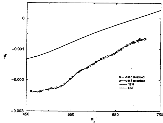
Figure B.9 Comparison of stretched grid to equidistant 12 \delta (32 points per \lambda_x , 10 points per \delta ).
