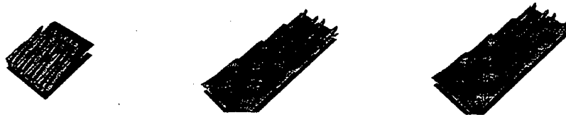
Figure 6.29 Oblique subharmonic resonance: Isosurface of spanwise vorticity \omega_z = 15 for cases I, II and III from left to right, respectively; Re = 10^5 , F_{2,x} = 5 \times 10^{-5} , F_{1,x} = 2.5 \times 10^{-5} , \Psi_{2,x} = 60^\circ
