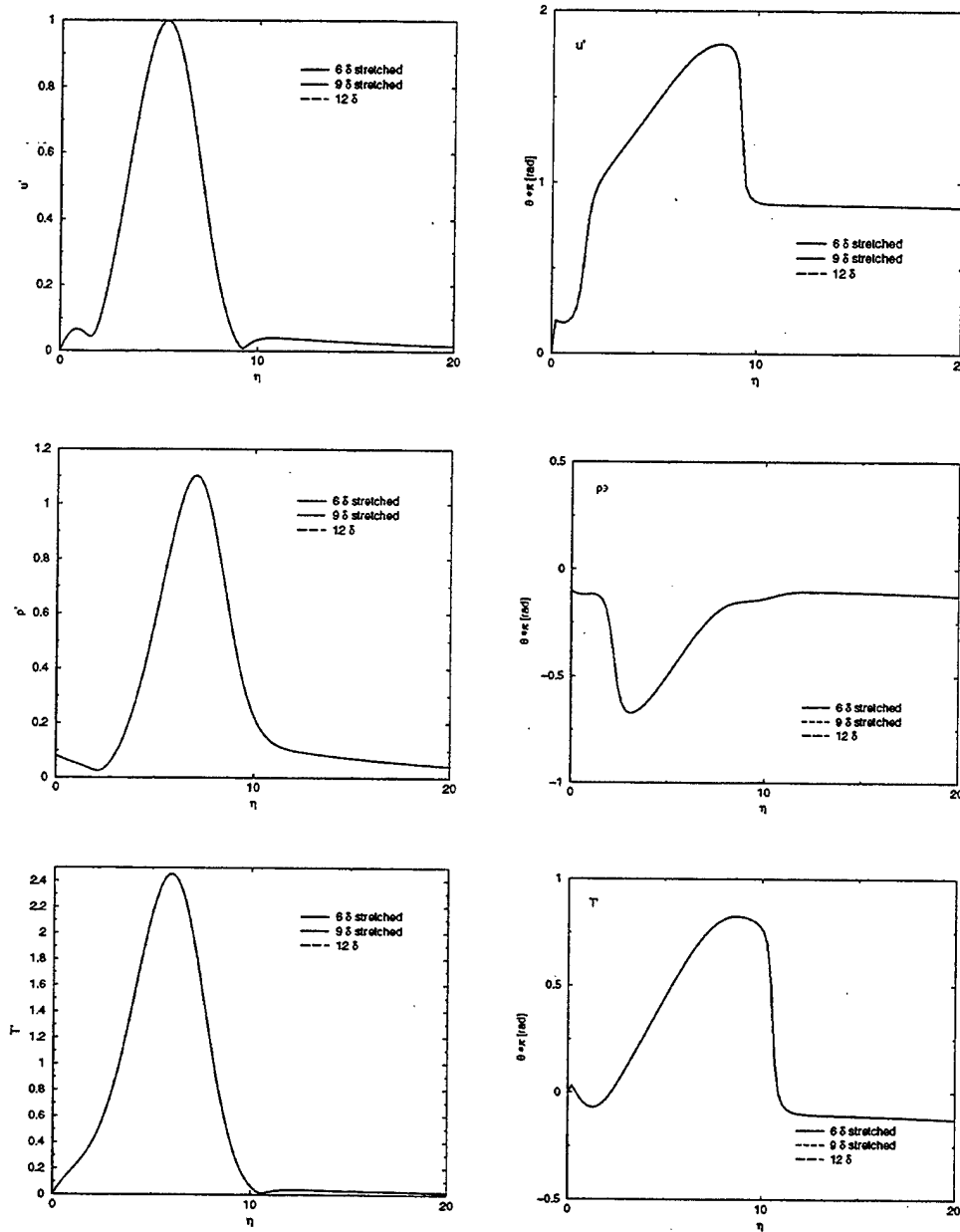
Figure B.10 Influence of the grid stretching on the amplitude distribution (left column) and phase (right column) of u' , \rho' and T' at Re_x = 500 (32 points per \lambda_x , 10 points per \delta ).
