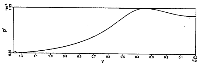
Figure 6.21 Pressure eigenfunction at R_x = 940 .
