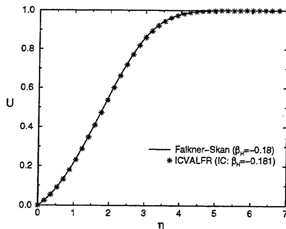
Figure 4.7 Comparison between Falkner-Skan solution and the baseflow obtained from DNS. The u -velocity profile is plotted over the similarity variable \eta .
