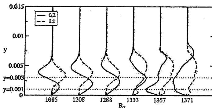
Figure 6.39 Development of the amplitude distribution of u_{[h,k]}/u_{[h,k]max} over y .
