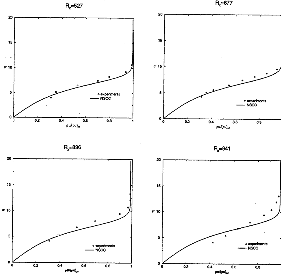
Figure 6.4 Comparison of computation and experiment at different downstream locations.
