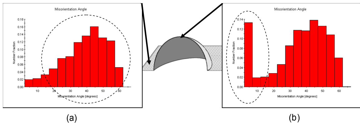
Figure 20 Histograms for 3 \times 10^{-4} \text{ s}^{-1} sample depicting (a) high-angle boundaries and (b) the occurrence of low-angle boundaries.
