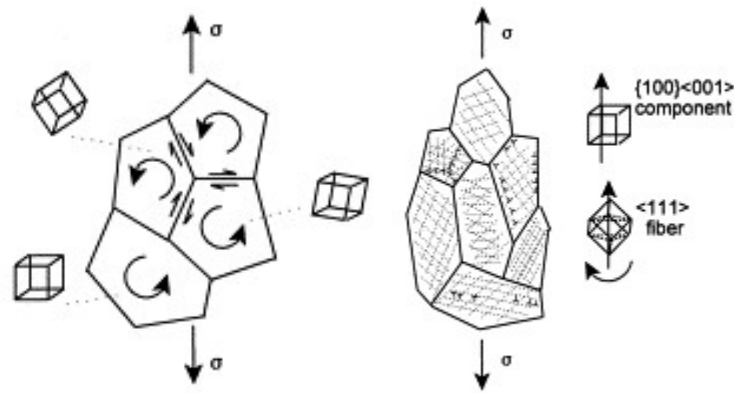
Figure 11 Schematics of the microstructural effect of (a) Grain Boundary Sliding and (b) Dislocation Creep ([From Ref. 17]).
