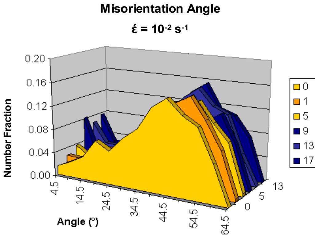
Figure 23 Misorientation angle distributions for 10^{-2} \text{ s}^{-1}
