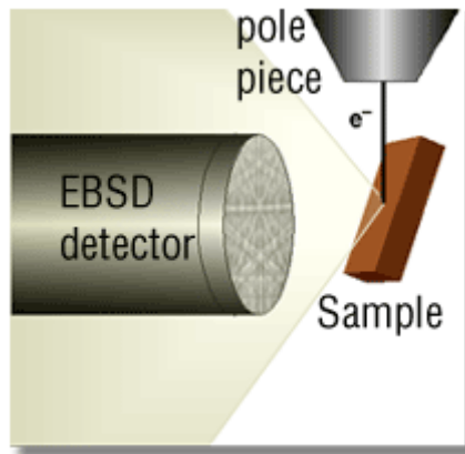
Figure 17 Electron backscatter diffraction schematic ([From Ref. 12]).
