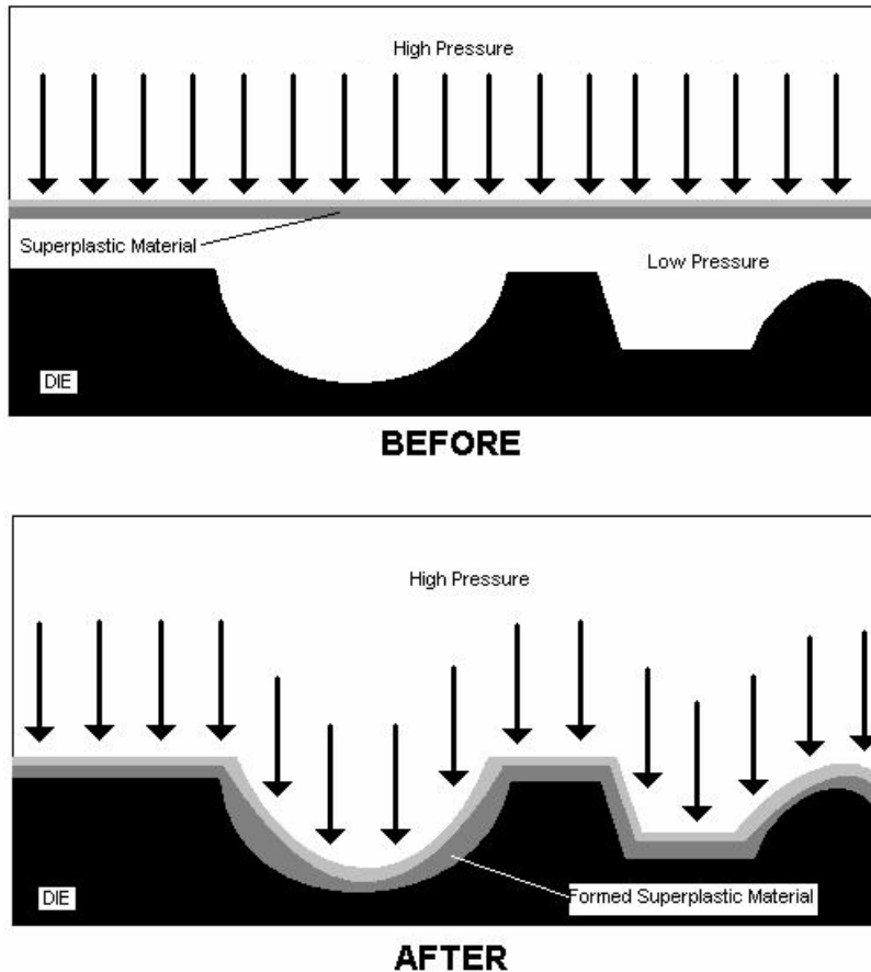
Figure 1: Schematic of Superplastic Forming Process ([From Ref. 5])
