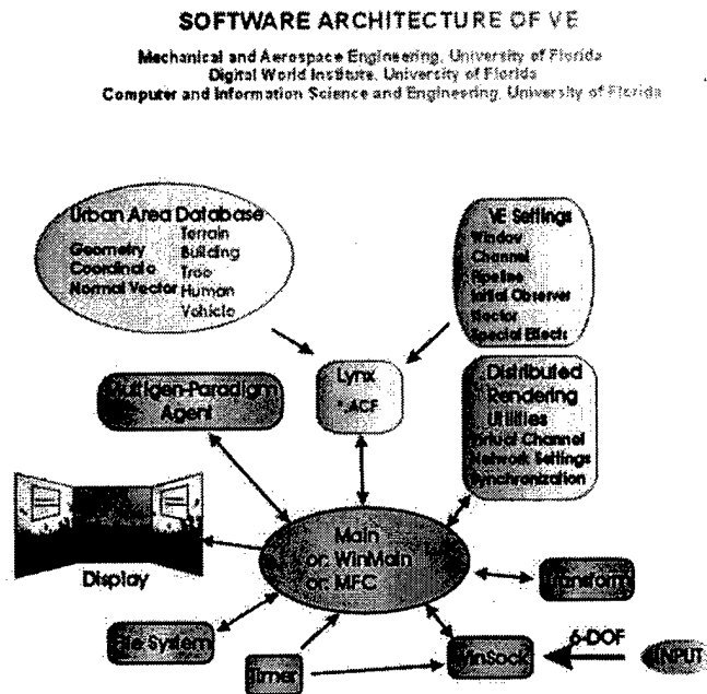
Figure 3: Software architecture of the visualization facility.
