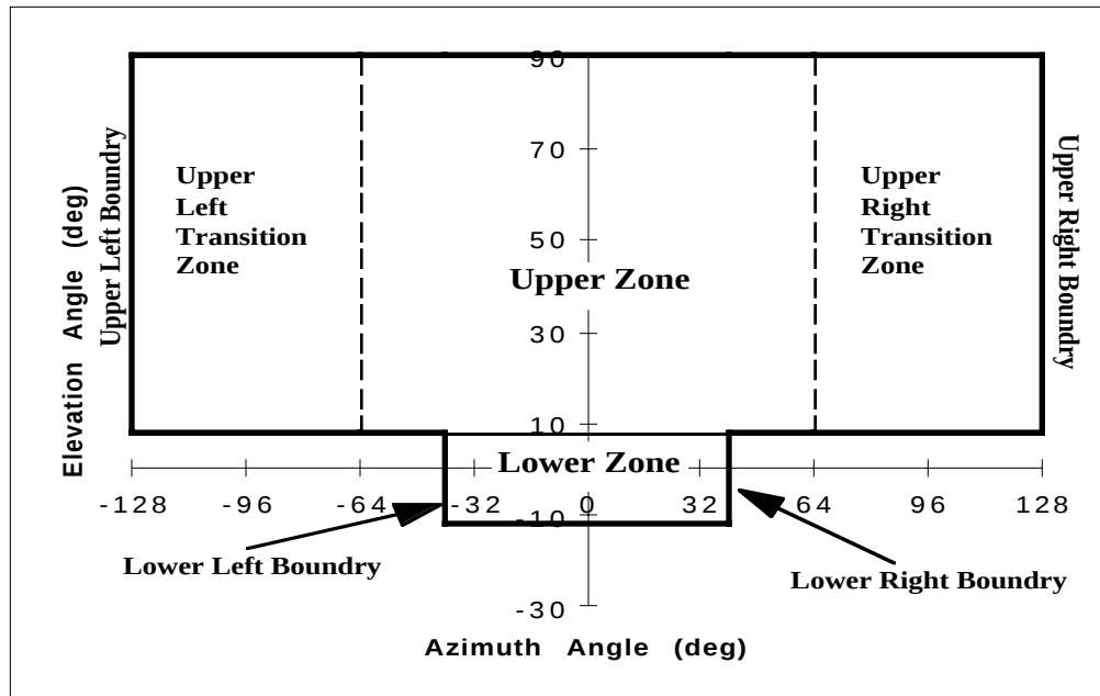
Figure 4. Zones in angle space over which the dual-zone angular deviation fit model is valid.
